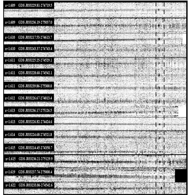
Fig. 8. Two dimensional spectra of 15 galaxies at z \sim 1.61 discovered in the RUN2. The [O II]3727 emission line is marked with vertical dashed lines around the 9727.5 \text{ \AA} position.
