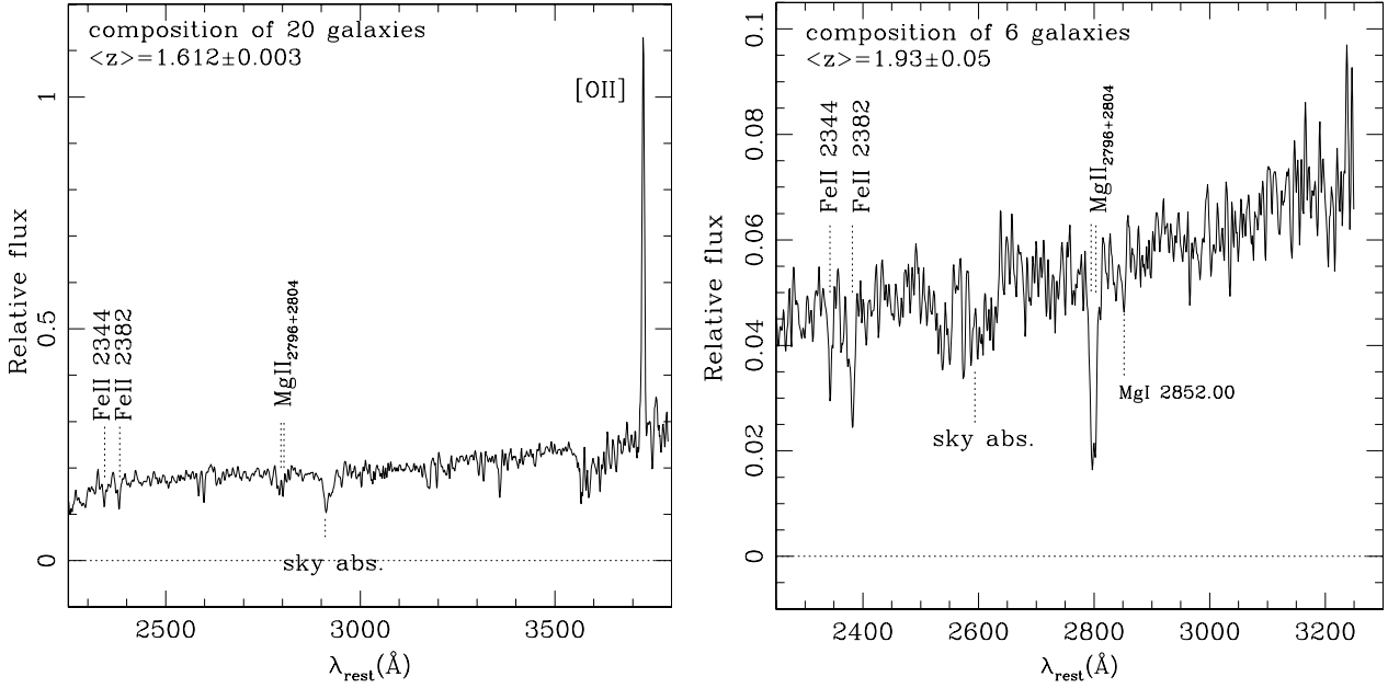
Fig. 9. Left panel: rest frame composite spectrum of 20 galaxies at redshift \sim 1.61 . The [O II]3727 is clearly evident and the Mg II 2798, 2802 \text{\AA} and [Fe II] 2344, 2383 \text{\AA} are also present. Right panel: rest frame composite spectrum of 6 galaxies at redshift \sim 1.93 .
