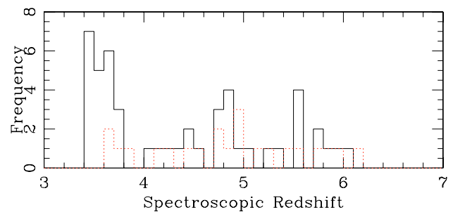
Fig. 5. Redshift distribution according to the selection functions described in Sect. 2 for the spectroscopic sample with quality A, B (solid line) and C (dotted line). In the top and bottom panels the sources at z < 2 ( dz = 0.04 ) and z > 2 ( dz = 0.1 ) are shown, respectively.
