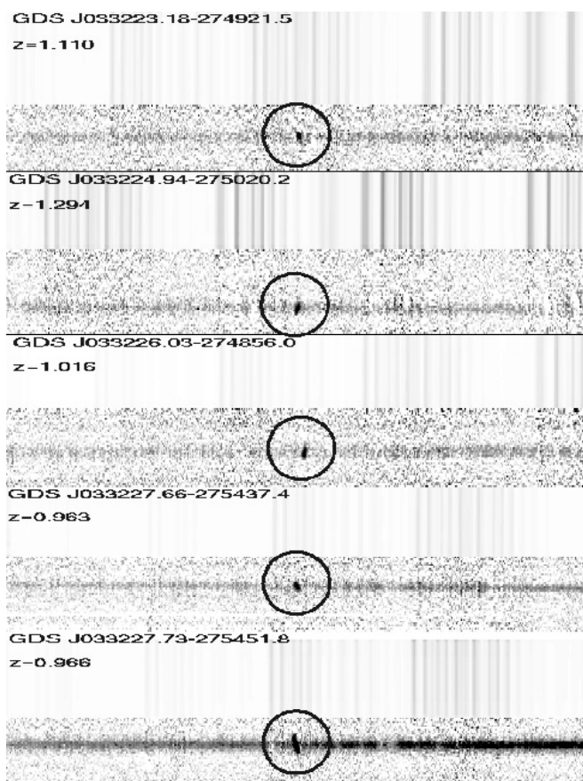
Fig. 15. An example of tilted [\text{O II}]3727 emission line (marked with a circle) at redshift around 1. The two dimensional FORS2 spectra are shown (object and sky lines).
