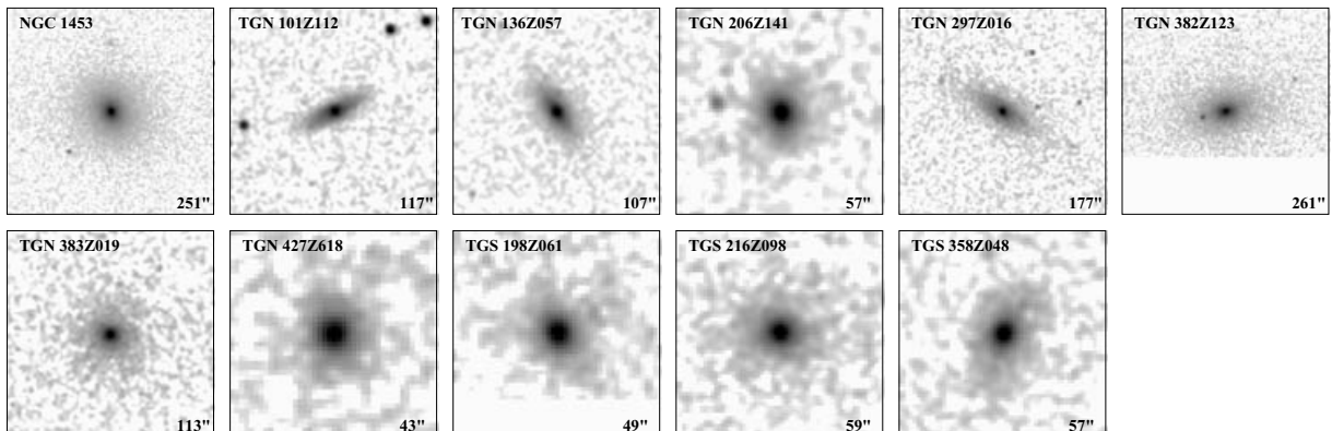
Figure 1. 2MASS ‘postage stamp’ J -band images for the 11 galaxies of the 2dFGRS sample. In each panel the size of the image is indicated in arcsec in the lower right, and north is up and east is left.
