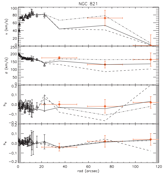
Figure 14. Best-fitting model for NGC 821 (bold line, M_{200} = 6.5 \times 10^{11} M_{\odot} ) compared to our data points at large radii (red filled circle) and the central SAURON data (open triangles). The dashed line indicates a model without halo and the dashed-dotted line a model with a too heavy halo ( M_{200} = 5.5 \times 10^{12} M_{\odot} ).
