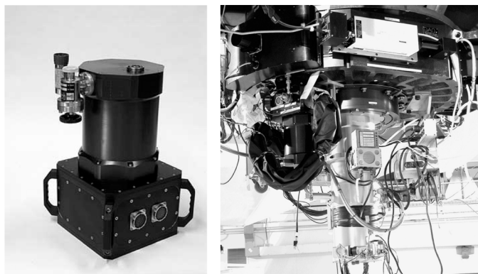
FIG. 3.— Left : FlyEyes dewar. Right : Mounted on PUEO (ringlike structure at the top) at the Cassegrain focus of CFHT; the dewar in the middle is the KIR scientific imaging camera. See the electronic edition of the PASP for a color version of this figure.
