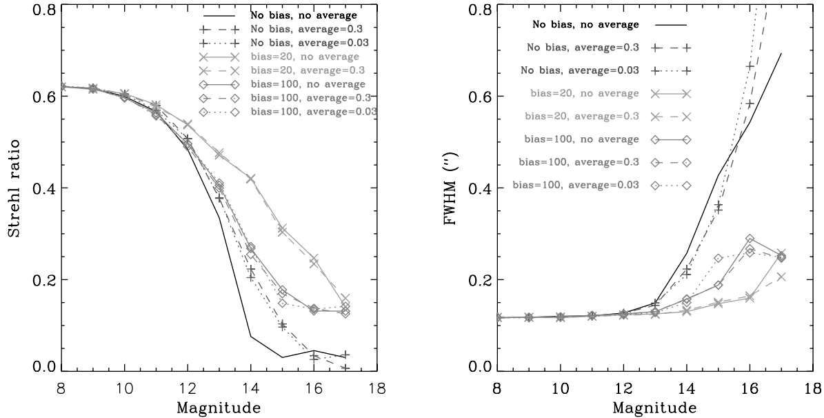
FIG. 7.—Simulated Strehl ratio and FWHM as a function of guide star magnitude, with bias or running average in denominator to prevent loop instabilities. A bias of 20 seems to provide the most improvement in this case.
