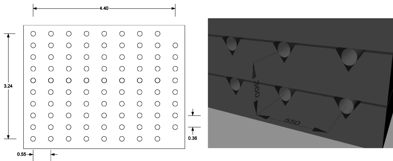
FIG. 4.— Left : Ferrule hole pattern (dimensions in millimeters); this method would have provided a more precise fiber bundle. Right : Illustration of the stacked silicon v-groove spacers. These ended being used because they had already been fabricated and were available. See the electronic edition of the PASP for a color version of this figure.
