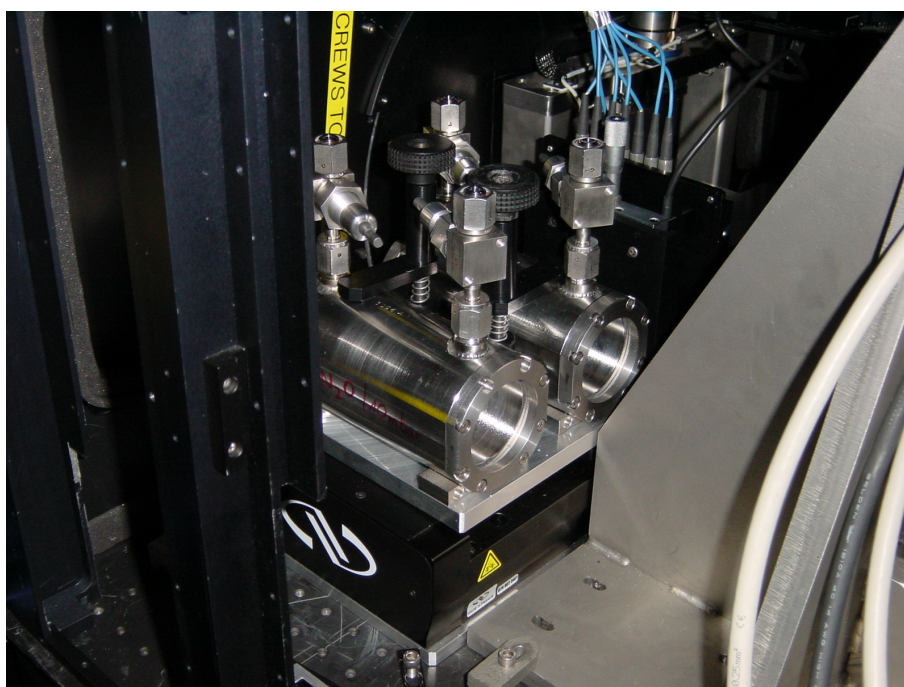
Figure 15: The N 2 O and CO gas-cells mounted on the carriage
