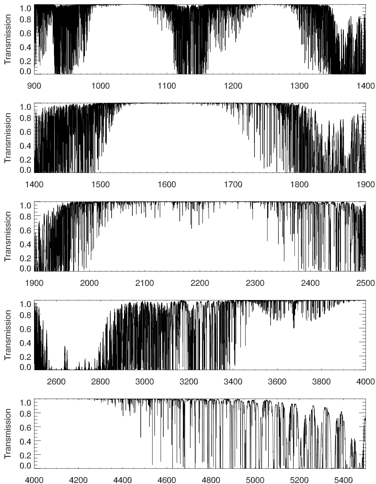
Figure 24: Atmospheric transmission from 900 – 5500nm computed with RFM/HITRAN for a Paranal atmosphere, precipitable water vapor (PWV) of 2.5mm, at zenith at a resolution of \lambda/\Delta\lambda = 100000 .
