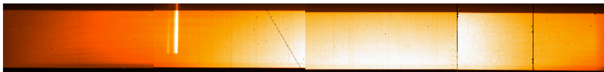
Figure 22: Example of a quasi-white light ghost observed with a reference wavelength of 1153.8 nm. The ghost is visible in staring frames top left on the second detector. Also, a diagonal (middle) and a vertical (right) detector scratches are also visible.
