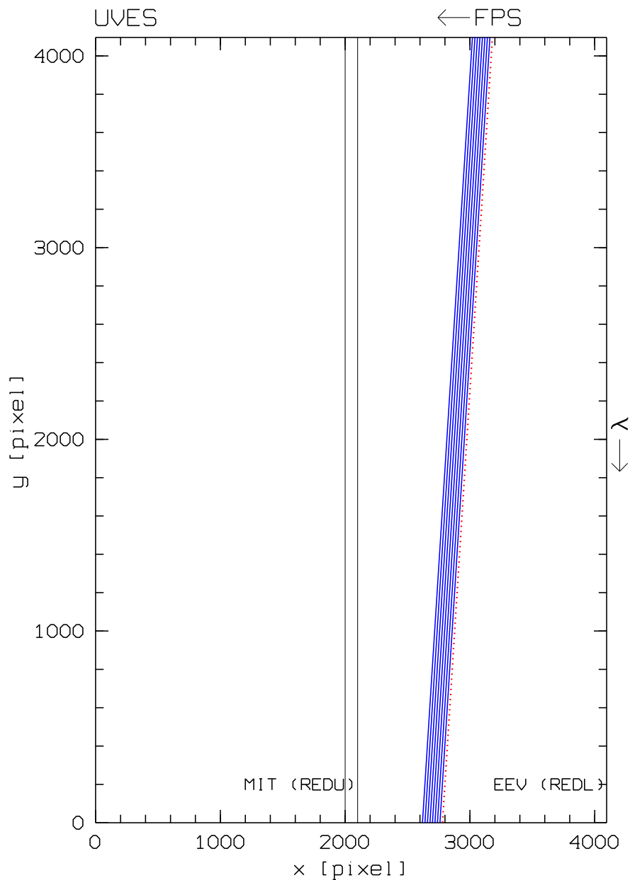
Figure 22: Schematic layout of the UVES – FIBRE spectral format for one order: blue solid lines: object fibres, red dots: calibration fibre. The direction of the increasing fibre number in the slit (FPS) and increasing wavelength \lambda are indicated. Redder echelle orders are to the left.
