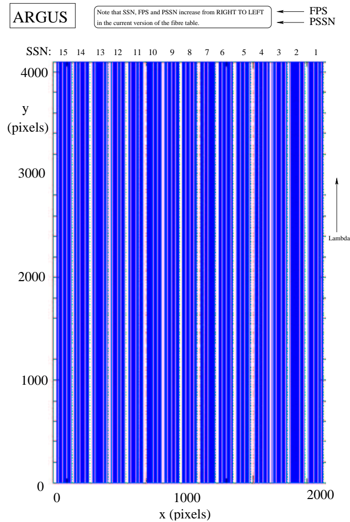
Figure 21: Schematic layout of the ARGUS spectral format: blue solid lines: object fibres, red dots: calibration fibres, green dots: sky fibres. The direction of the increasing fibre number in the slit (FPS) and increasing wavelength \lambda are indicated. Note that the directions of FPS, SSN and PSSN are inverted w.r.t. MEDUSA and IFU.
