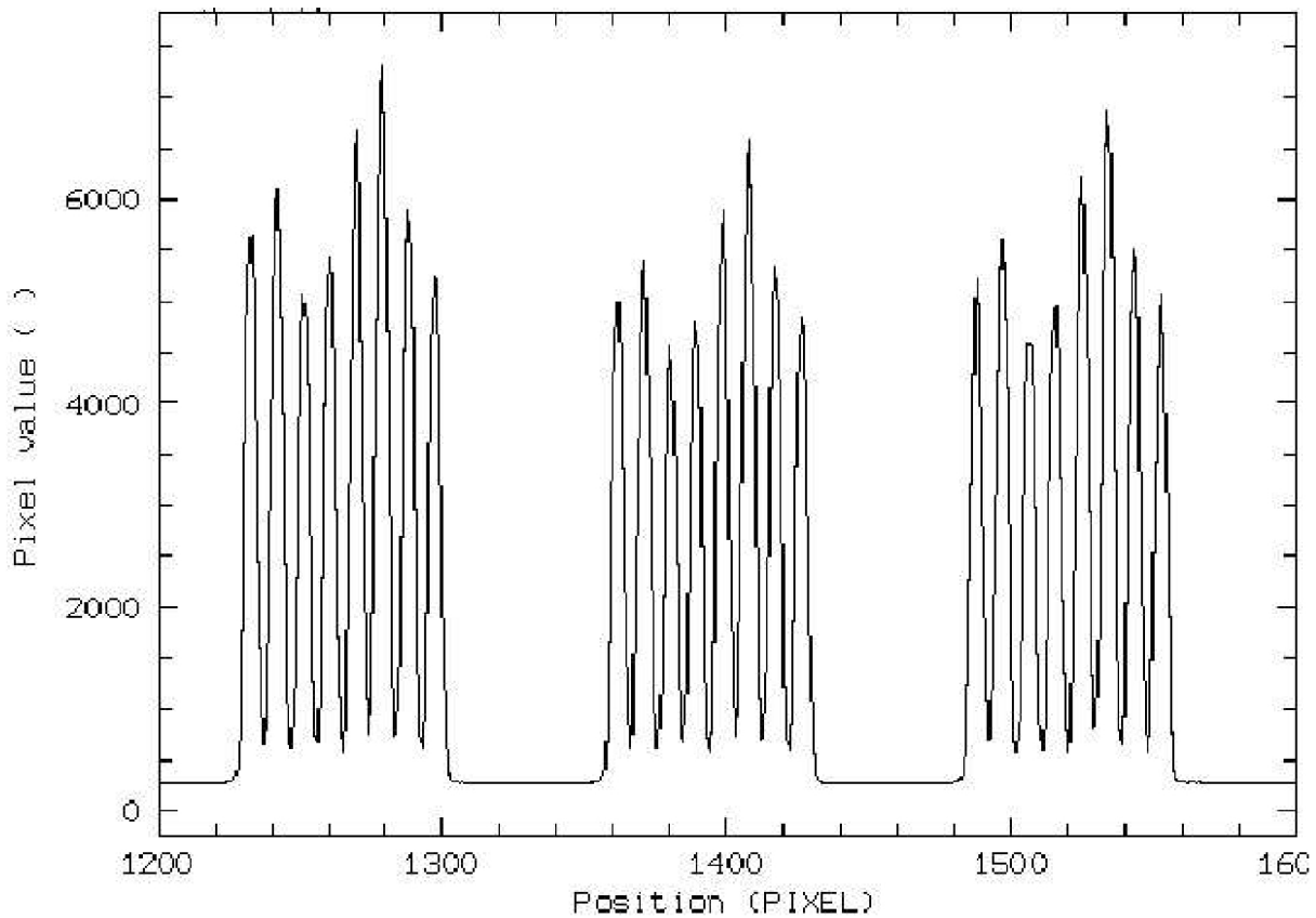
Figure 13: This figure shows a trace perpendicular to the dispersion of an UVES-FIBRE frame, containing three orders. Note the slight flux overlap between contiguous fibres. the UVES-Fibre data reduction software is designed to deblend the contributions
