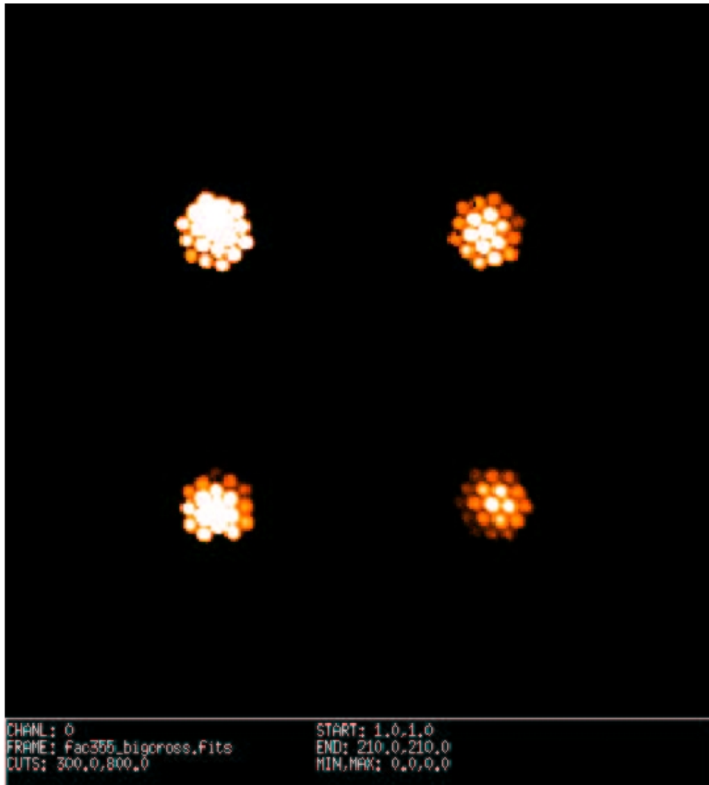
Figure 4: Image of Four fiducial stars as seen in the Technical CCD through the 4 Fiducial Acquisition Bundles (FACBs). Each bundle is composed of 19 ordered fibres, which image the star on 4 quadrants of the TCCD.
