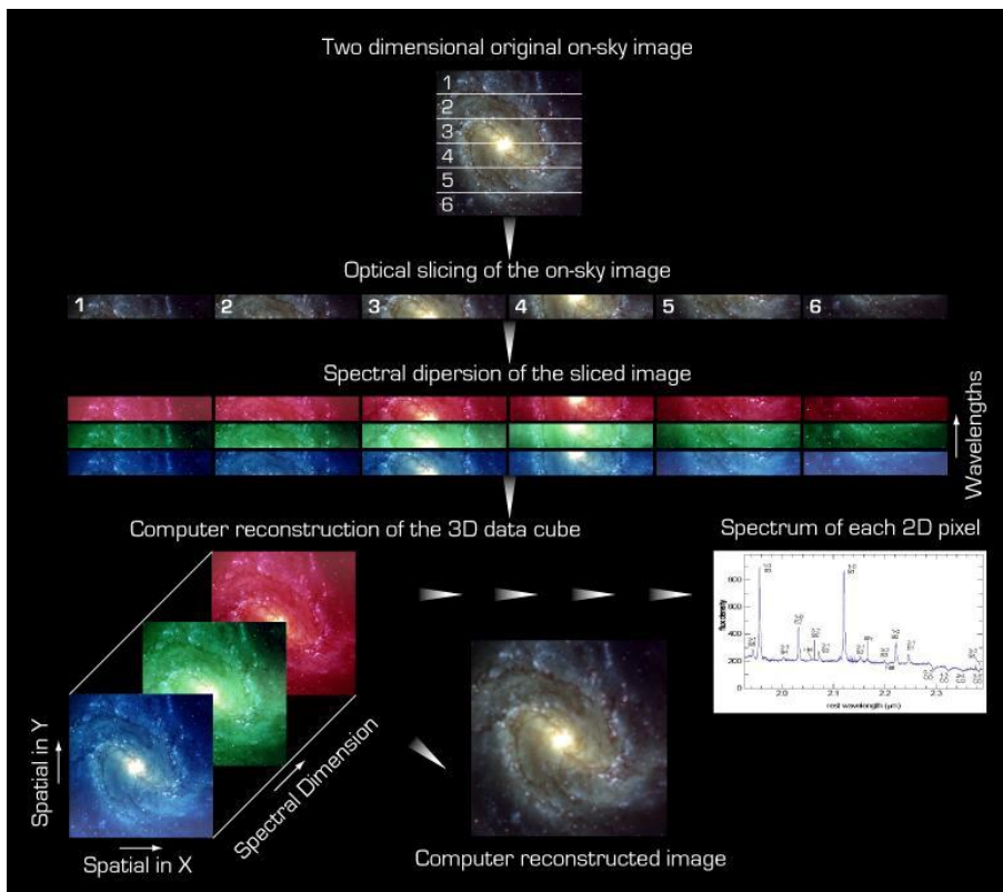
Figure 4: The function of the image slicer. The field of view (top) is slit into small slices which are recombined into a pseudo longslit before being dispersed. The dispersed planes can be recombined to an image, or used to extract spectra at a given point in the field of view.
