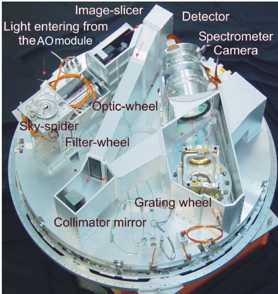
Figure 13: An inside view of SPIFFI: The cryostat cover and the reinforcing structure have been removed to provide a free view on the opto-mechanical components of SPIFFI. The light enters from the top, and passes the sky-spider. The pre-optics with a filter-wheel and interchangeable lenses provides three different image scales. The image slicer re-arranges the two-dimensional field into a pseudo-long slit, which is perpendicular to the base plate. Three diamond turned mirrors collimate the light onto the gratings. In total, four gratings are implemented on the grating drive. A multiple-lens system then focuses the spectra on a Rockwell HAWAII array. The diameter of the instrument is 1.3m.
