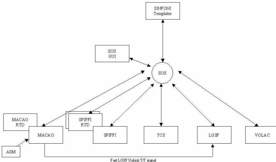
Figure 17: SINFONI software overview
