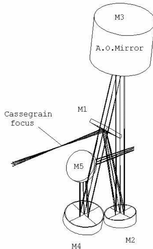
Figure 6: Main optics
