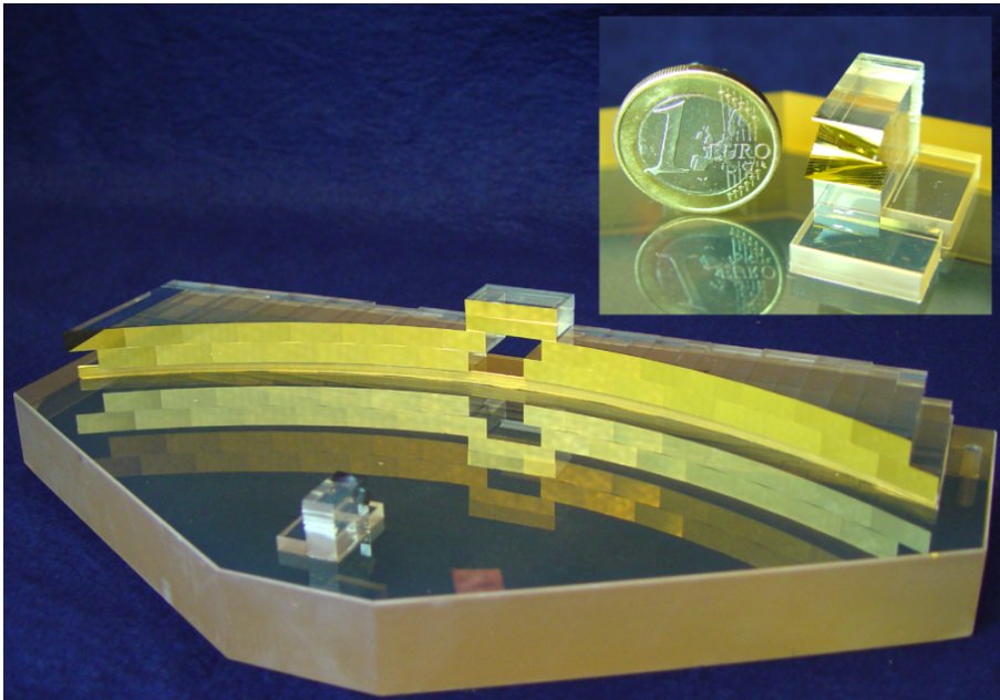
Figure 14: SPIFFI image slicer (a): The light enters through the hole in the big slicer. A stack of 32 small mirrors, the small slicer (also shown in the sub-panel), slices the image and redirects the light towards the 32 mirrors of the big slicer, which re-arranges the slitlets into a 31 cm long pseudo-slit.
