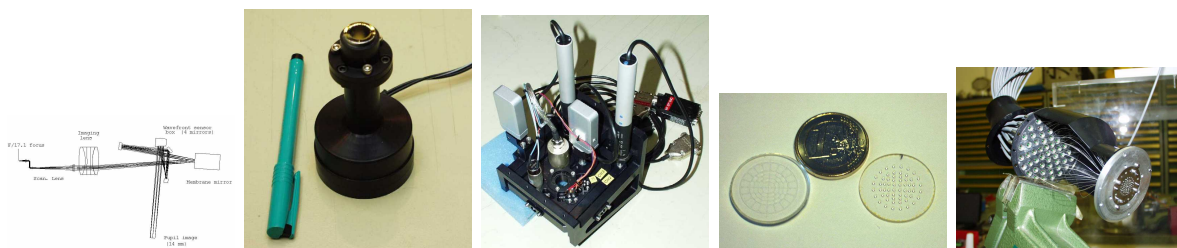
Figure 8: WFS optics – Membrane mirror – Gimbal mount – Lenslet array – Fiber module
