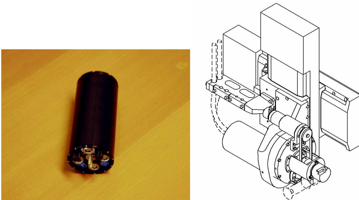
Figure 9: STRAP unit – STRAP assembly
