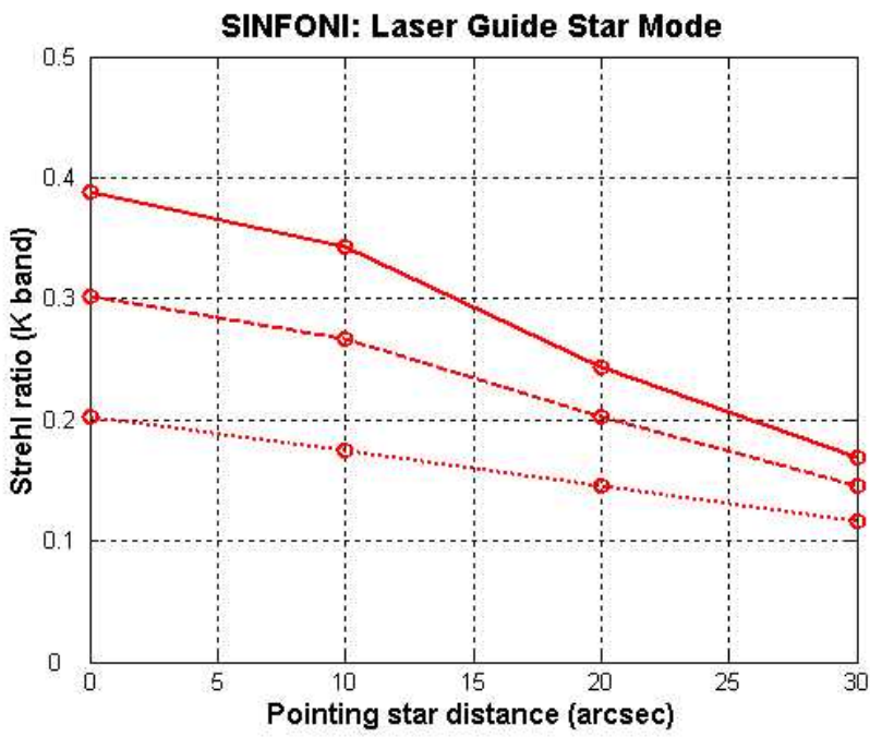
Figure 12: LGS Strehl performance
