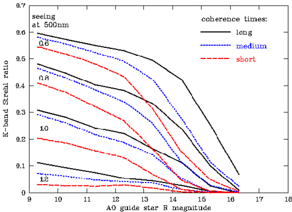
Figure 11: NGS performance for a wide range of optical seeing values (0.6 to 1.2'' ) and long, medium and short coherence times.
