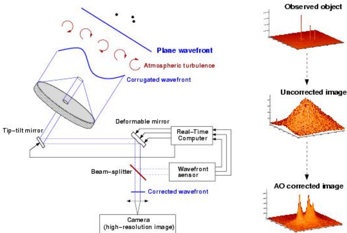
Figure 2: Principle of Adaptive Optics. Note that in practice, and contrary to this schematic design, SINFONI has no dedicated Tip-Tilt mirror, but performs low- and high-order corrections with a single deformable mirror (mounted on a tip-tilt stage).
