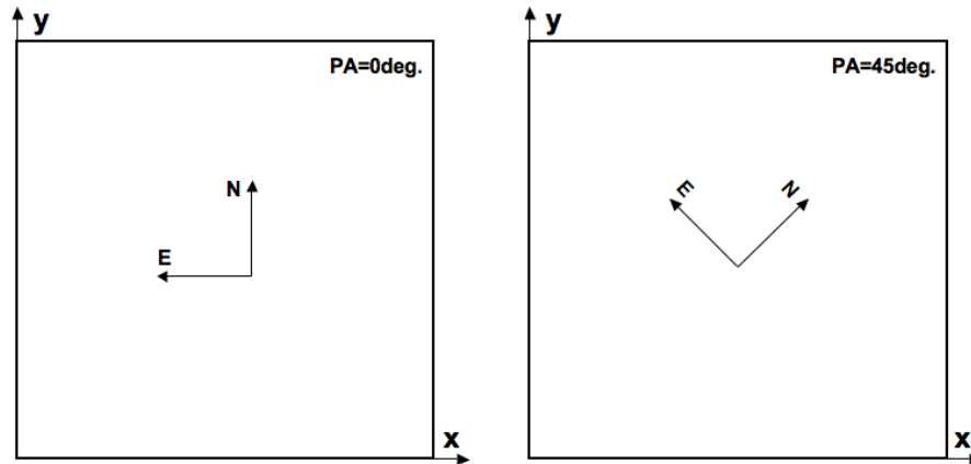
Figure 2: Illustration of the orientation convention of the Position Angle on Sky for a PA of 0deg. (left) and +45deg. (right).
