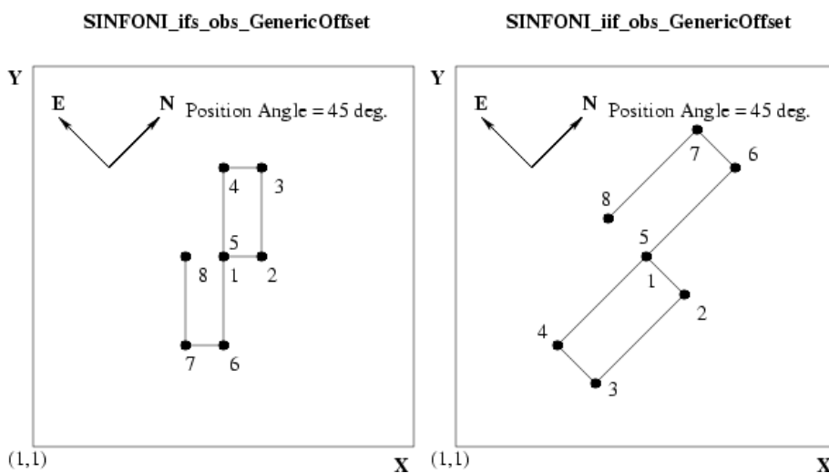
Figure 20: An illustration of the offset sequence taken with the GenericOffset template. Left side: Offset coordinate type "DETECTOR"; Right side: Offset coordinate type "SKY".
