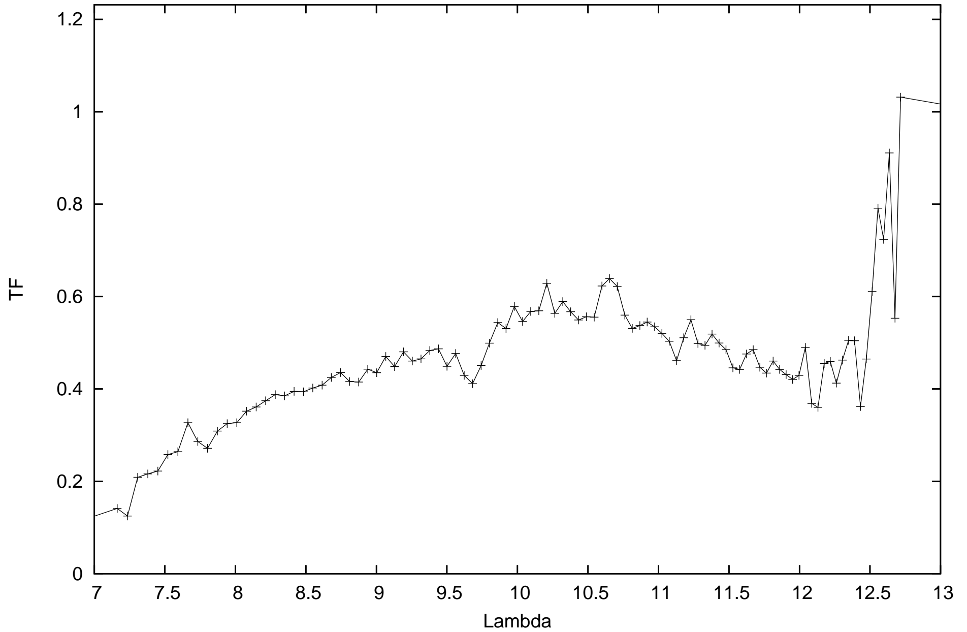
calhd1038_flux-9.9E+100_diam5.23_r.MIDI.2008-10-01T07_15_48.000_HIGHSENS
