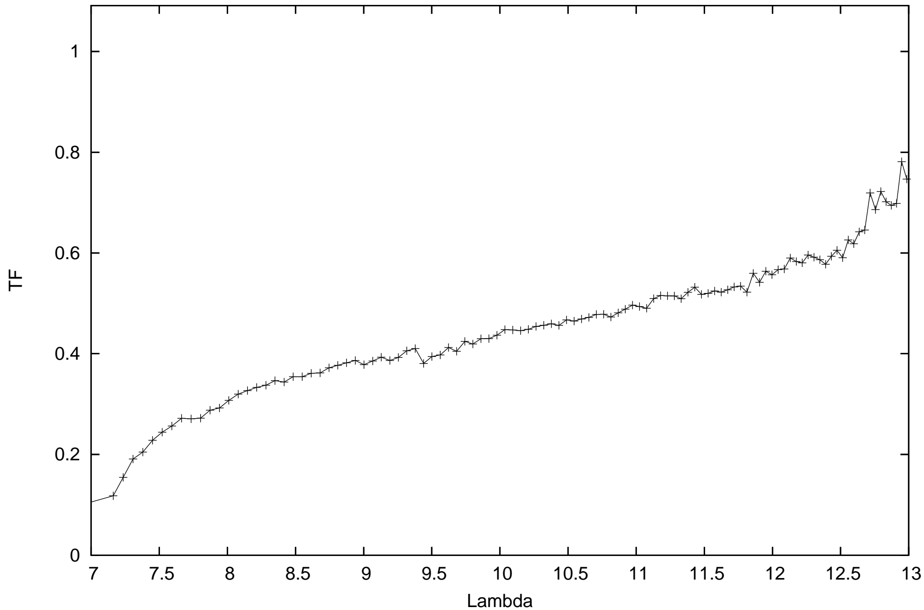
calhd167618_flux-9.9E+100_diam11.86_r.MIDI.2008-10-01T01_05_53.000_HIGHSENS
