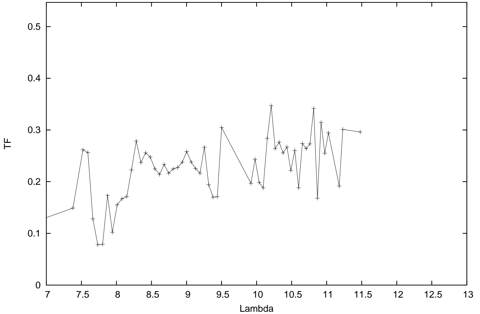
calhd183439_flux-9.9E+100_diam4.06_r.MIDI.2008-10-01T02_06_46.000_HIGHSENS
