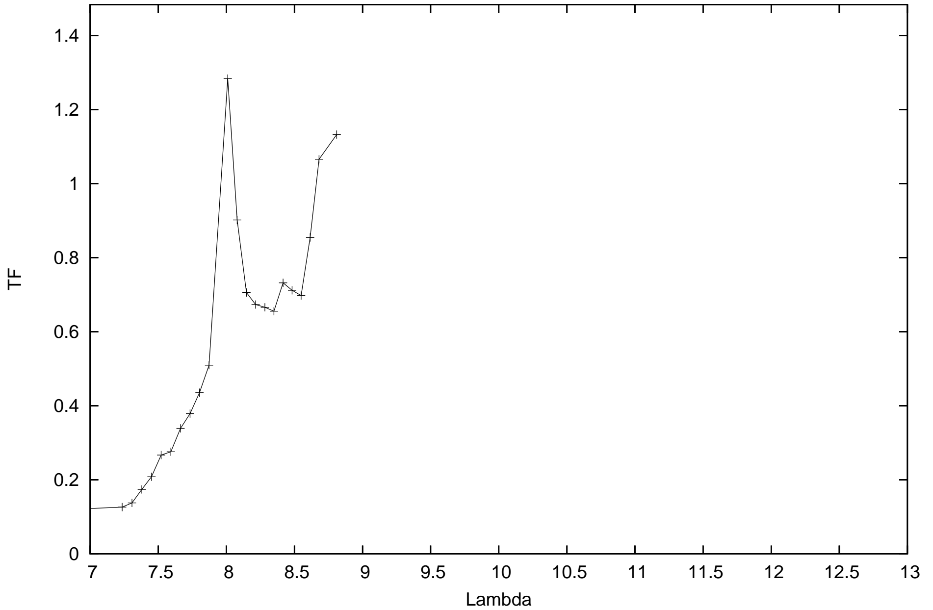
calhd202369_flux-9.9E+100_diam4.69_r.MIDI.2008-10-01T02_55_05.000_HIGHSENS
