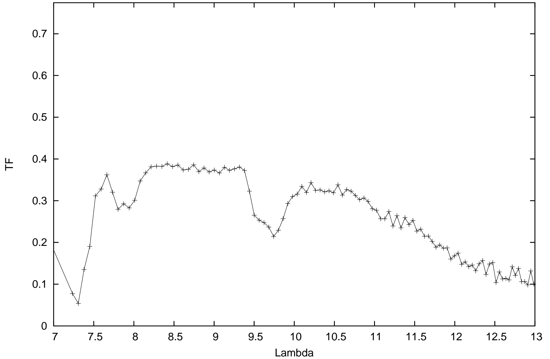
calHD004128_flux-0.44_diam5.23_r.MIDI.2008-11-03T02_58_13.000_HIGHSENS
