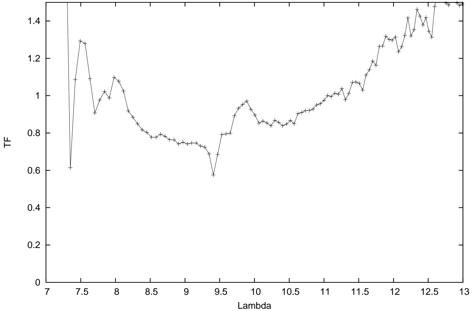
calHD040808_flux1.31_diam2.43_r.MIDI.2008-12-13T05_54_39.015 SCIPHOT
