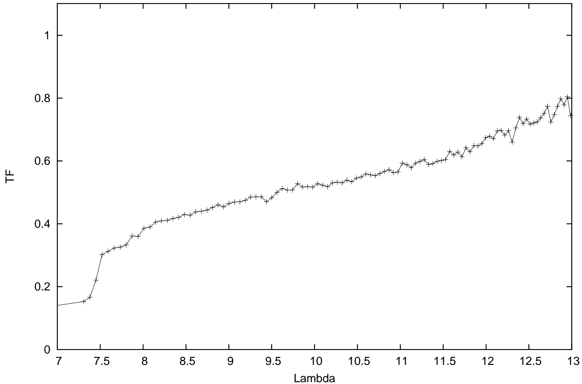
calHD048433_flux1.68_diam2.13_r.MIDI.2008-12-13T07_27_33.000_HIGHSENS
