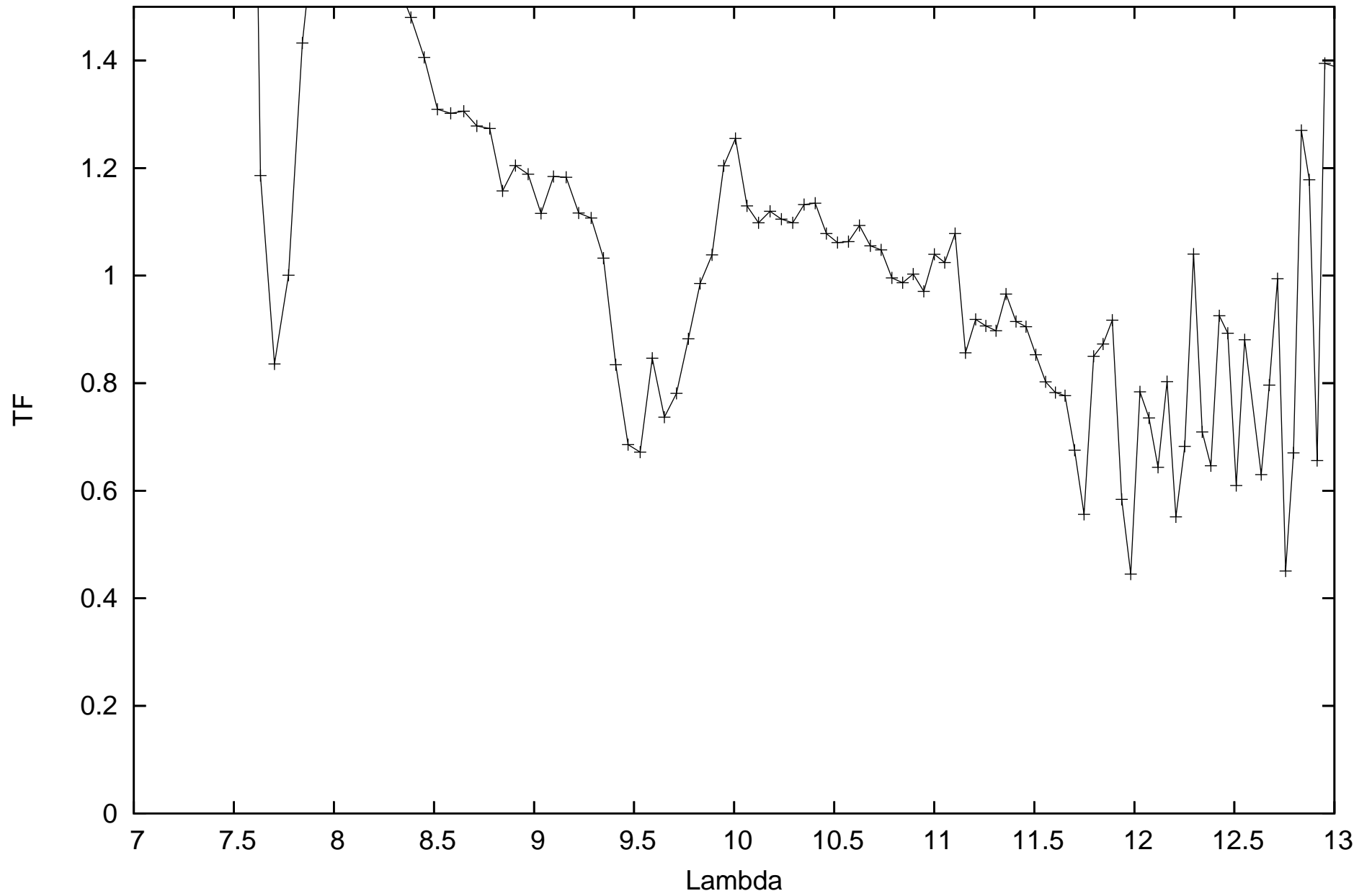
calHD224935_flux-0.85_diam7.24_r.MIDI.2008-12-28T01_21_18.179 SCIPHOT
