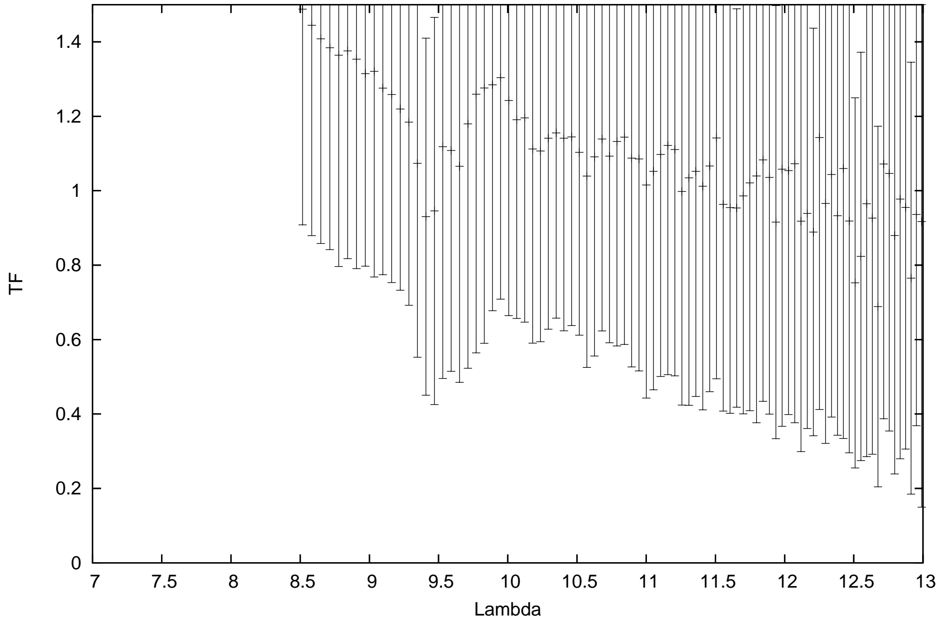
calHD224935_flux-0.85_diam7.24_r.MIDI.2009-01-01T00_37_04.180 SCIPHOT
