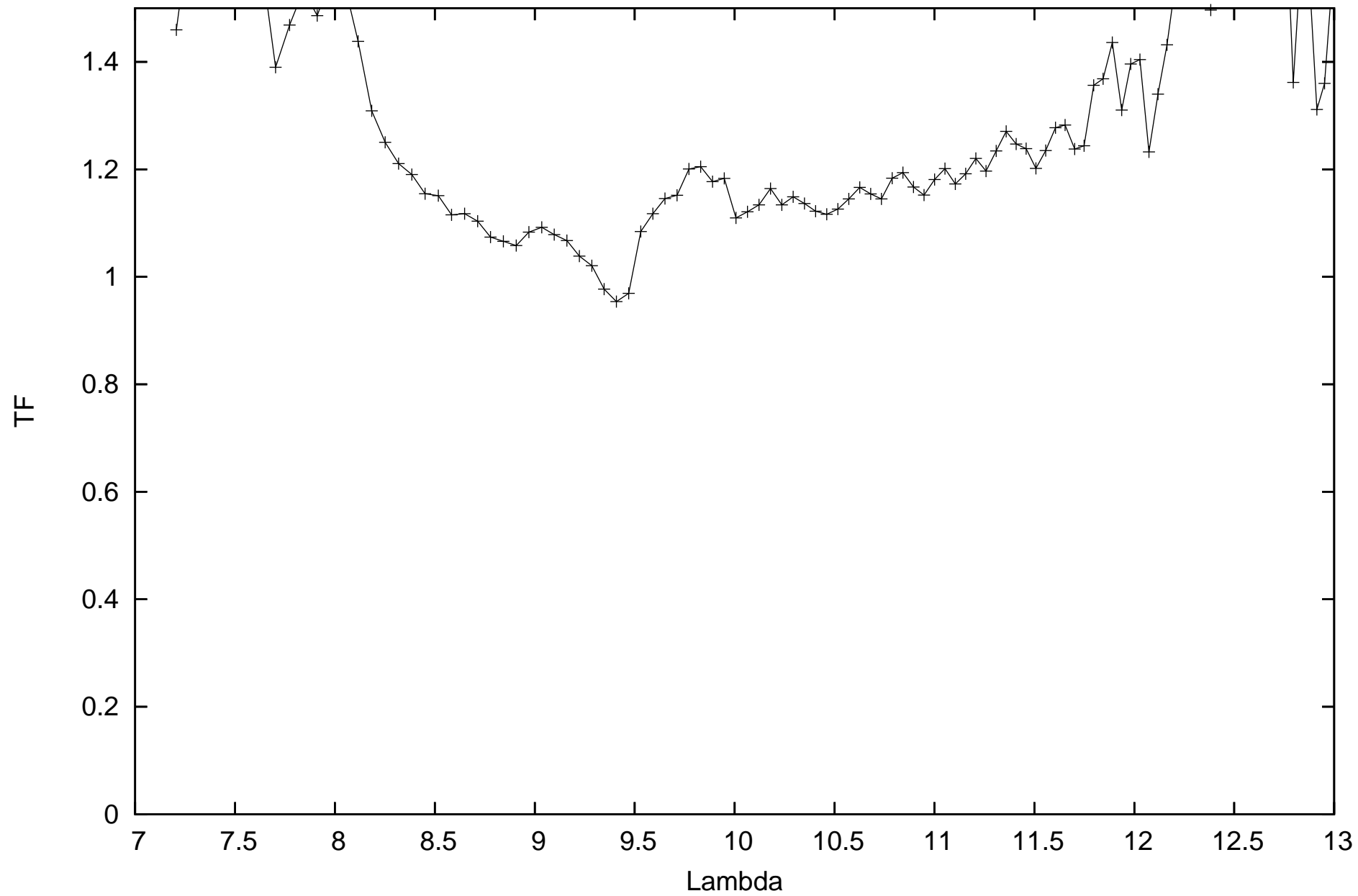
calHD081797_flux-1.49_diam9.14_r.MIDI.2009-01-16T06_40_58.179 SCIPHOT
