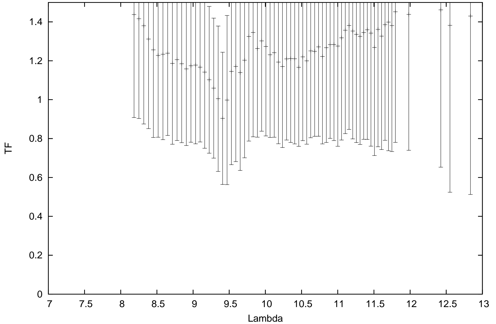
calHD081797_flux-1.49_diam9.14_r.MIDI.2009-01-19T06_23_06.959 SCIPHOT
