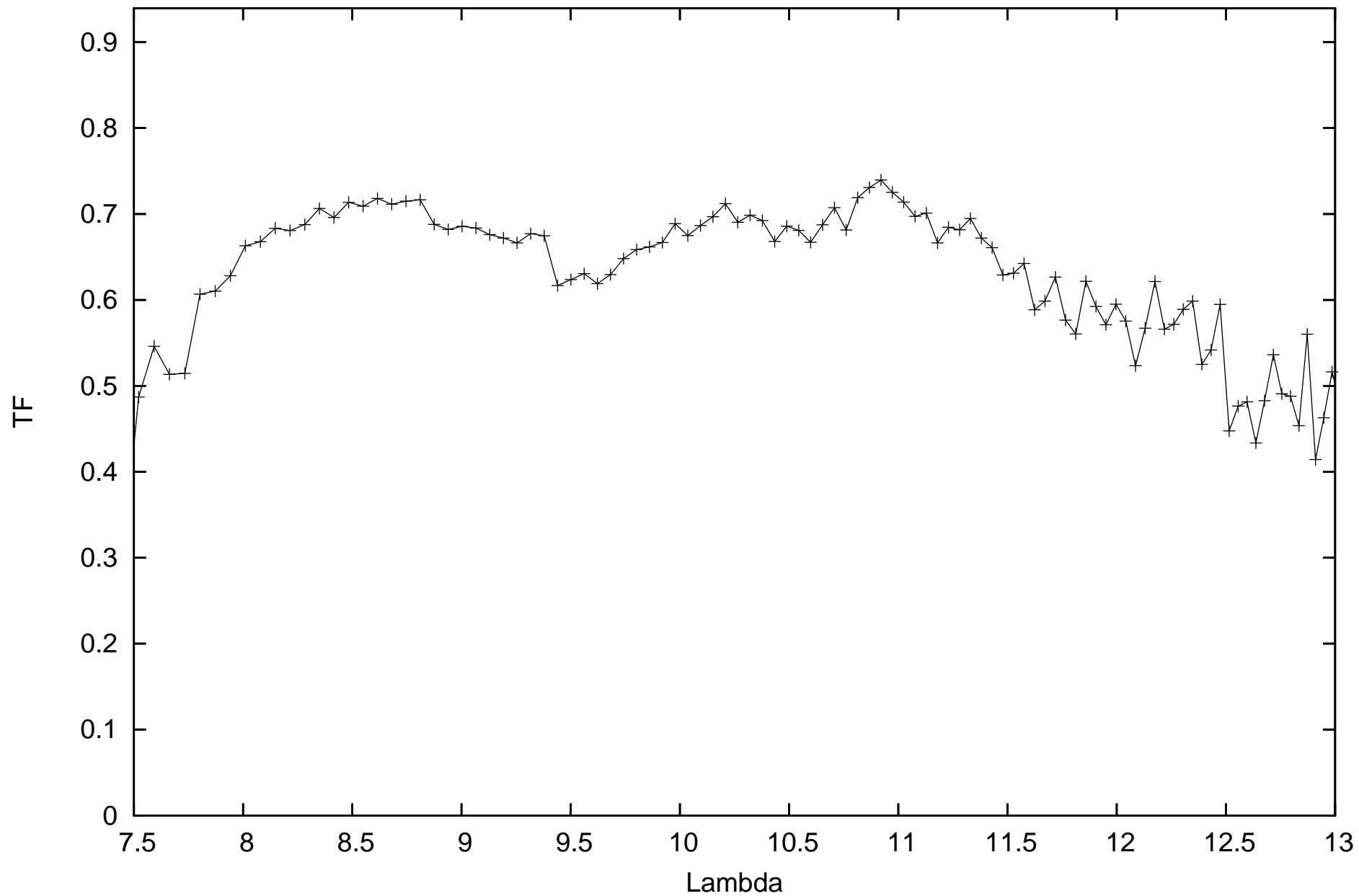
calHD107446_flux0.22_diam4.43_r.MIDI.2009-04-23T03_47_08.000_HIGHSENS
