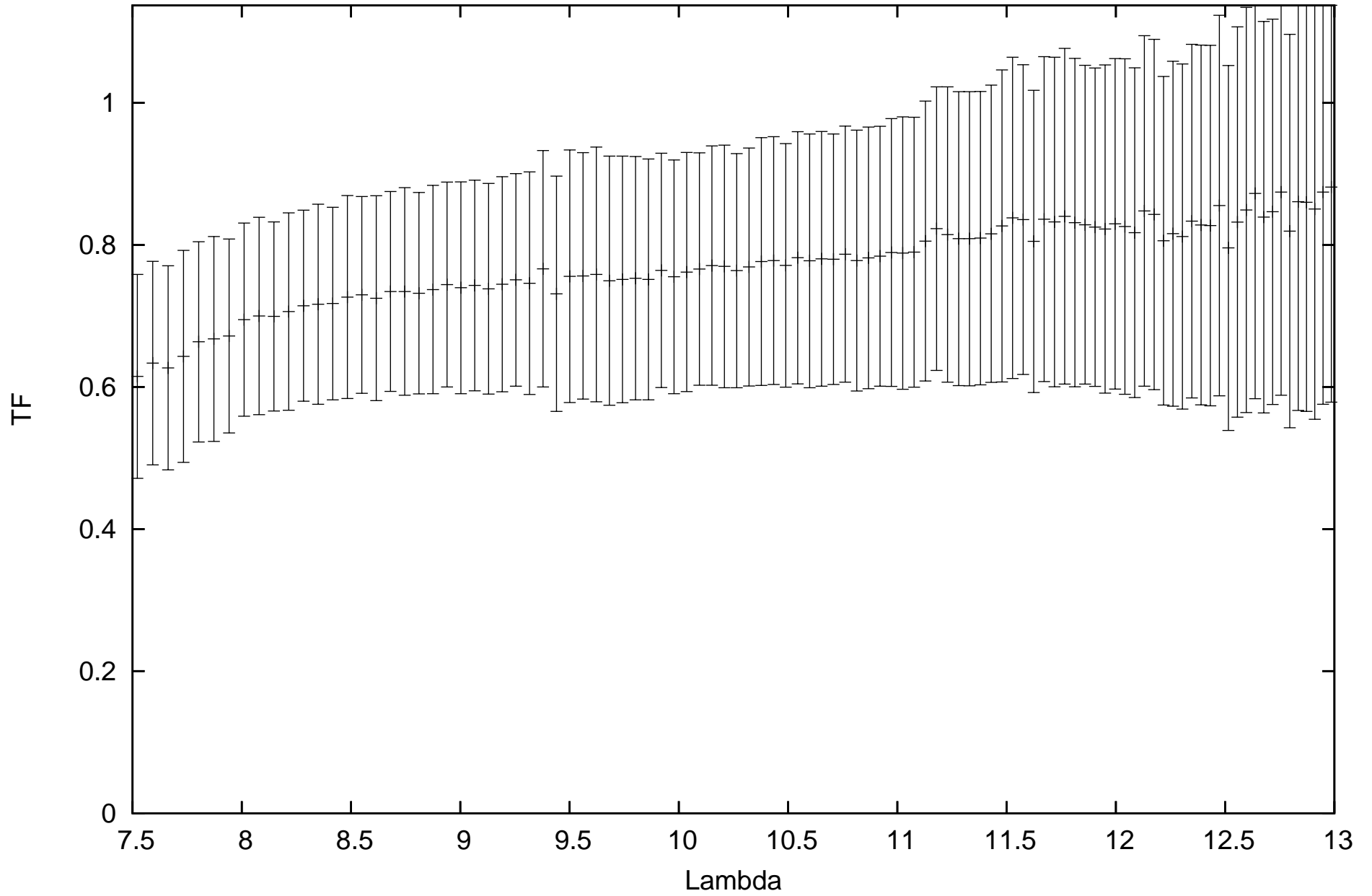
calHD167618_flux-1.82_diam11.66_r.MIDI.2009-04-23T09_09_48.000_HIGHSENS
