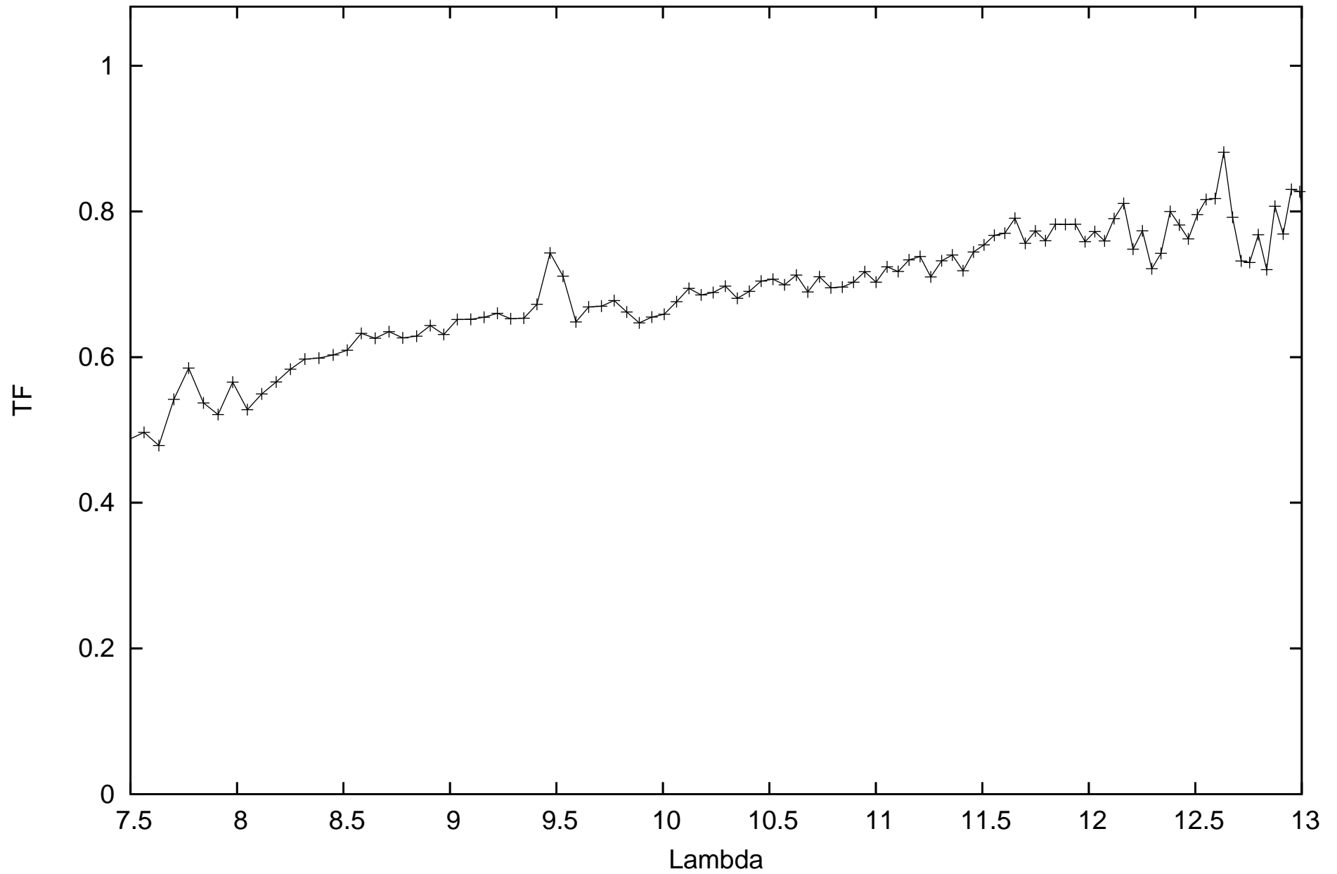
calHD167618_flux-1.82_diam11.66_r.MIDI.2009-04-23T09_18_32.137 SCIPHOT
