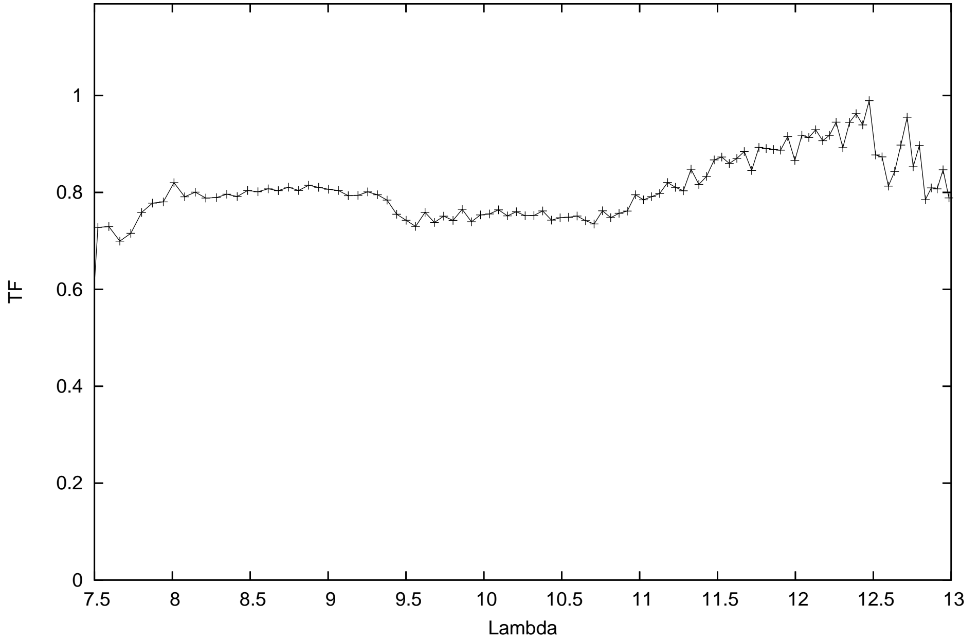
calHD089388_flux-0.2_diam5.18_r.MIDI.2009-04-24T02_16_35.000_HIGHSENS
