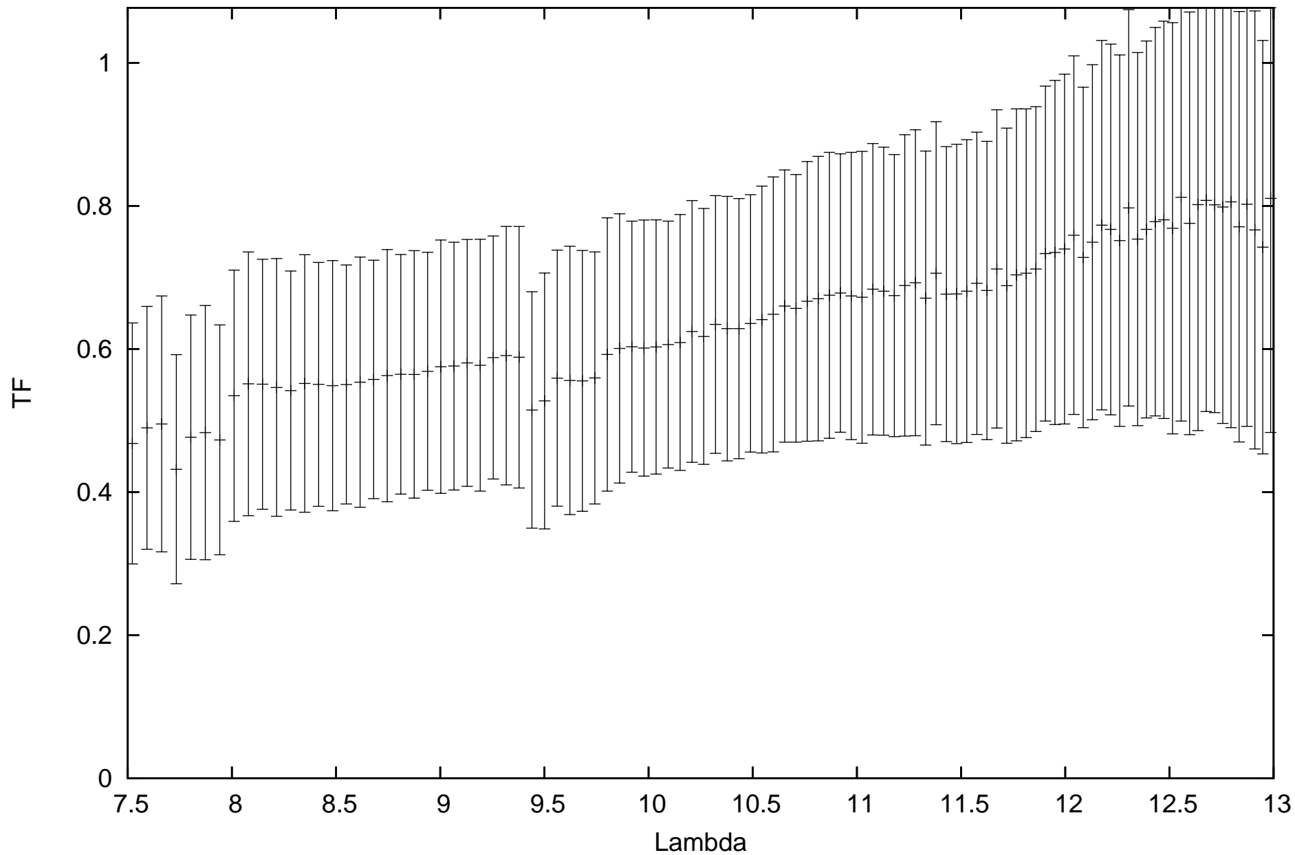
calHD150798_flux-1.4_diam8.91_r.MIDI.2009-04-27T10_28_55.000_HIGHSENS
