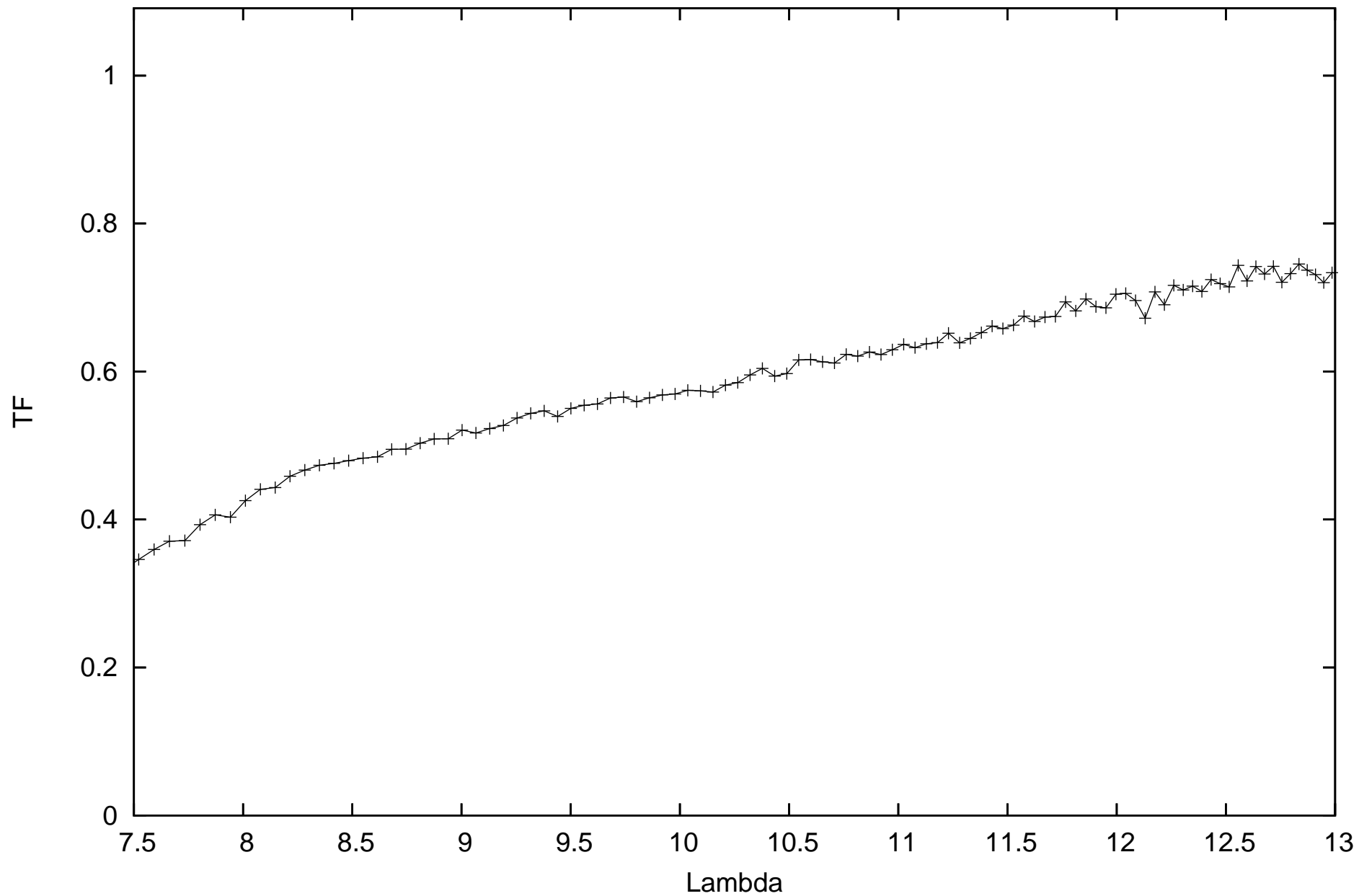
calHD112213_flux1.03_diam3.16_r.MIDI.2009-05-10T05_15_45.000_HIGHSENS
