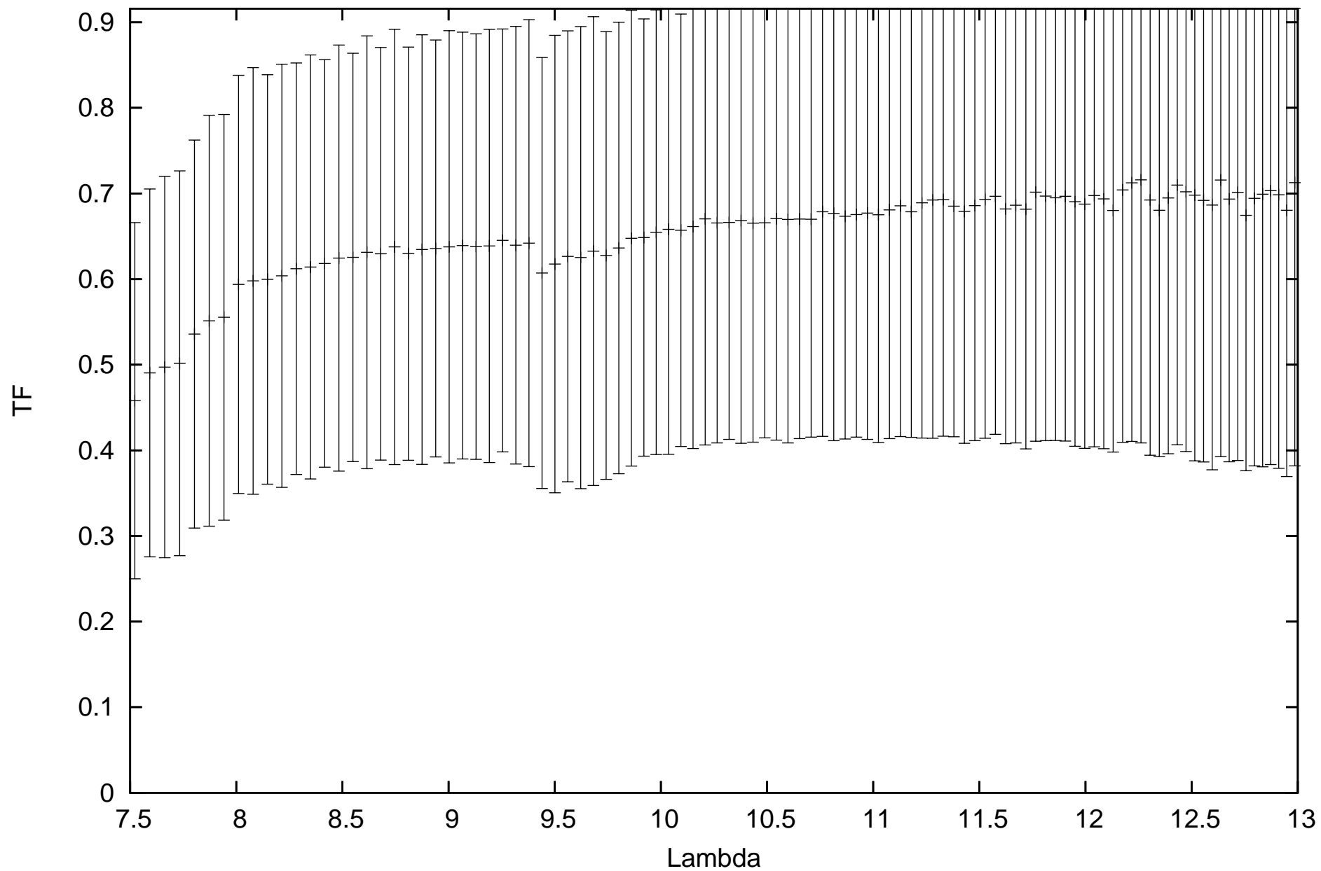
calHD112213_flux1.03_diam3.16_r.MIDI.2009-05-10T06_34_00.000_HIGHSENS
