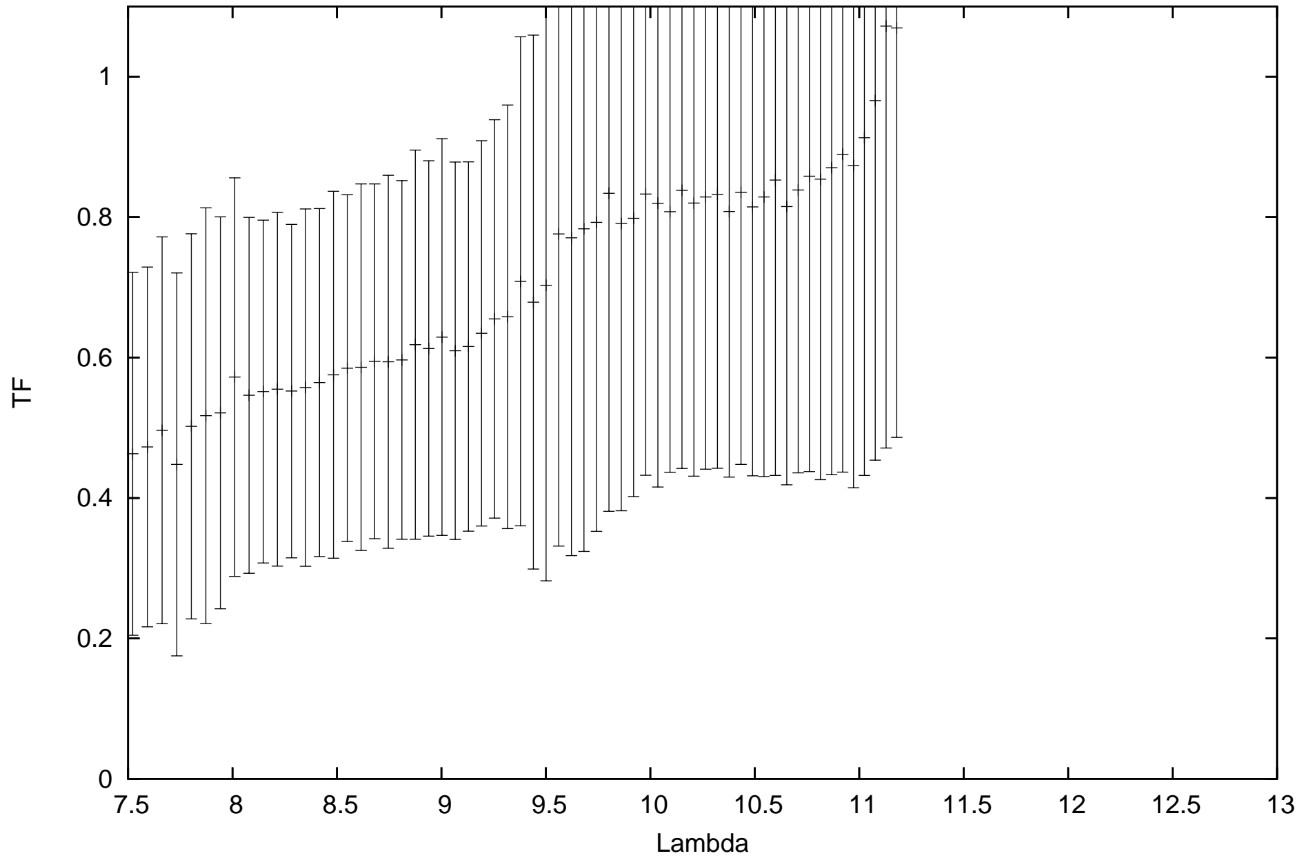
calHD107446_flux0.22_diam4.43_r.MIDI.2009-07-06T23_00_31.000_HIGHSENS
