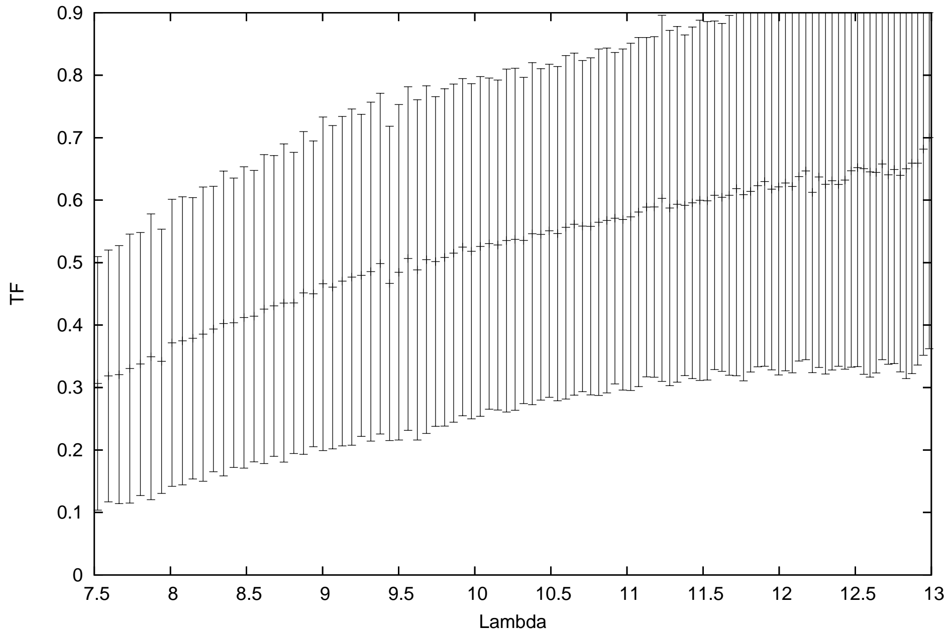
calHD167618_flux-1.82_diam11.66_r.MIDI.2009-10-20T01_57_48.000_G1H0
