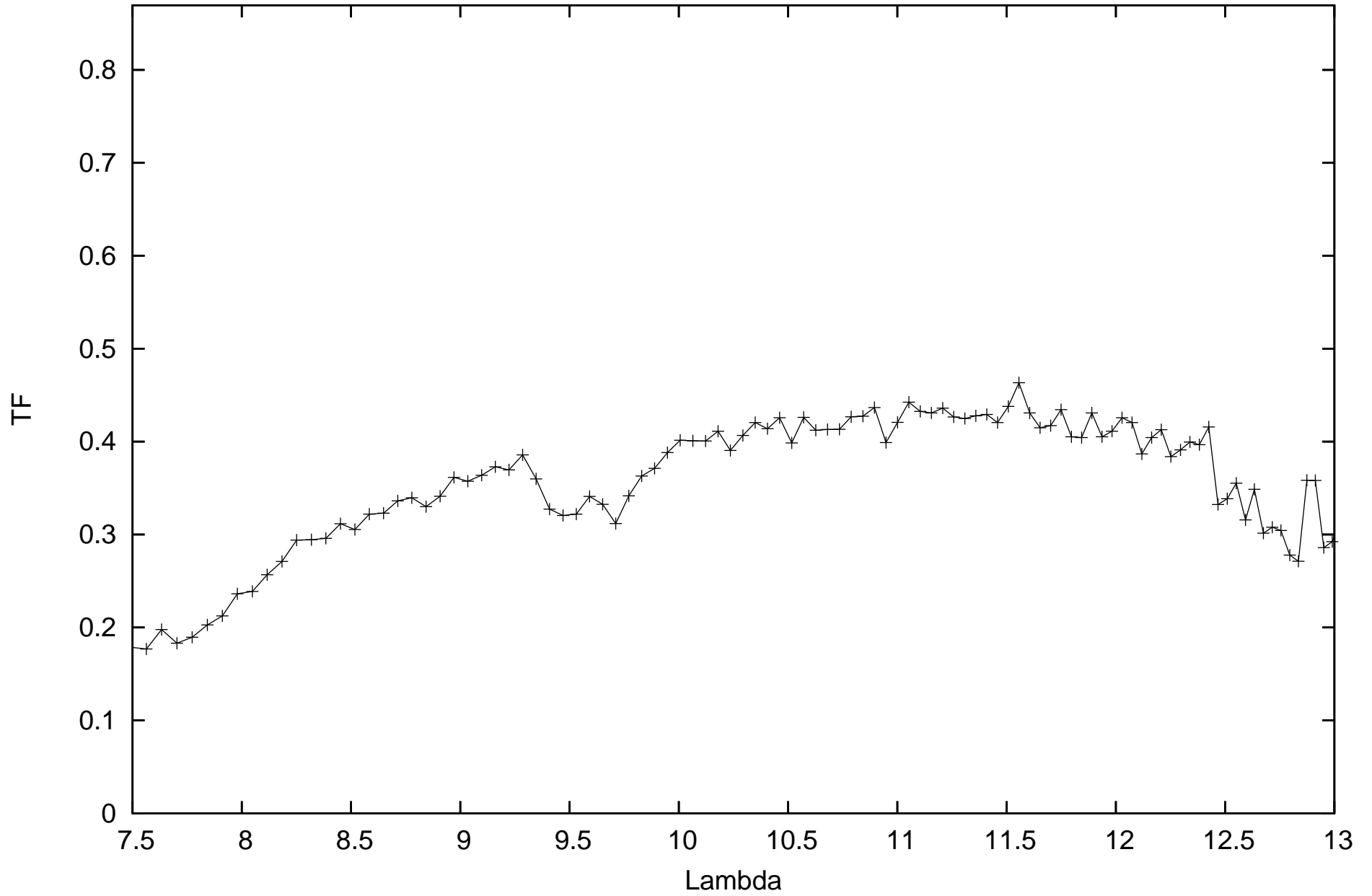
calHD224935_flux-0.85_diam7.24_r.MIDI.2009-10-21T04_46_26.522_H0D0
