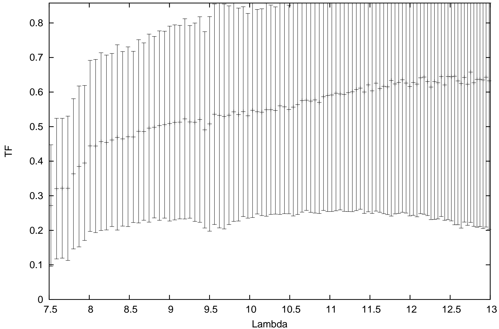
calHD023319_flux1.78_diam1.94_r.MIDI.2009-12-03T05_32_22.000_U2U4
