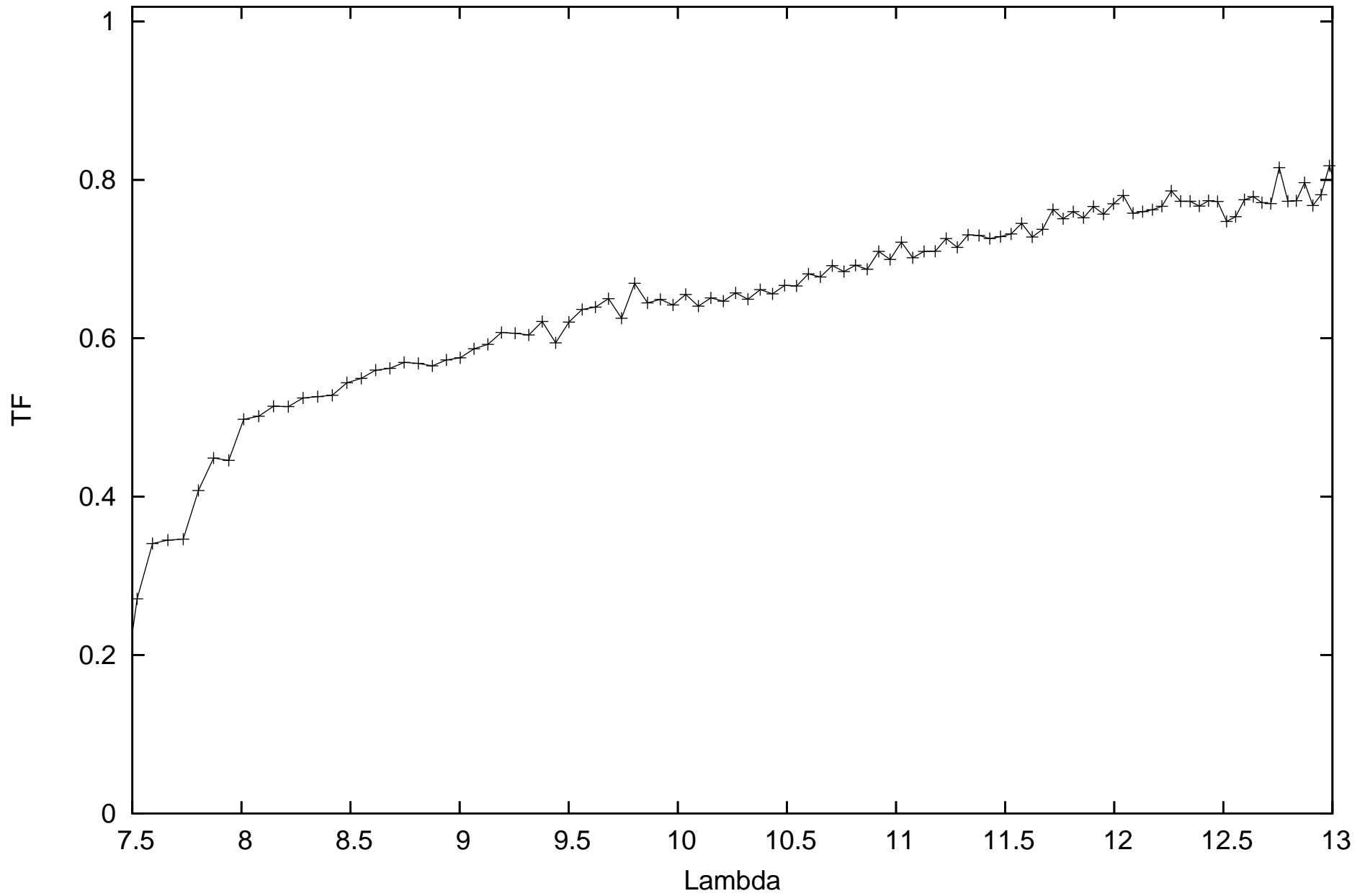
calHD023319_flux1.78_diam1.94_r.MIDI.2009-12-03T07_06_39.000_U2U4
