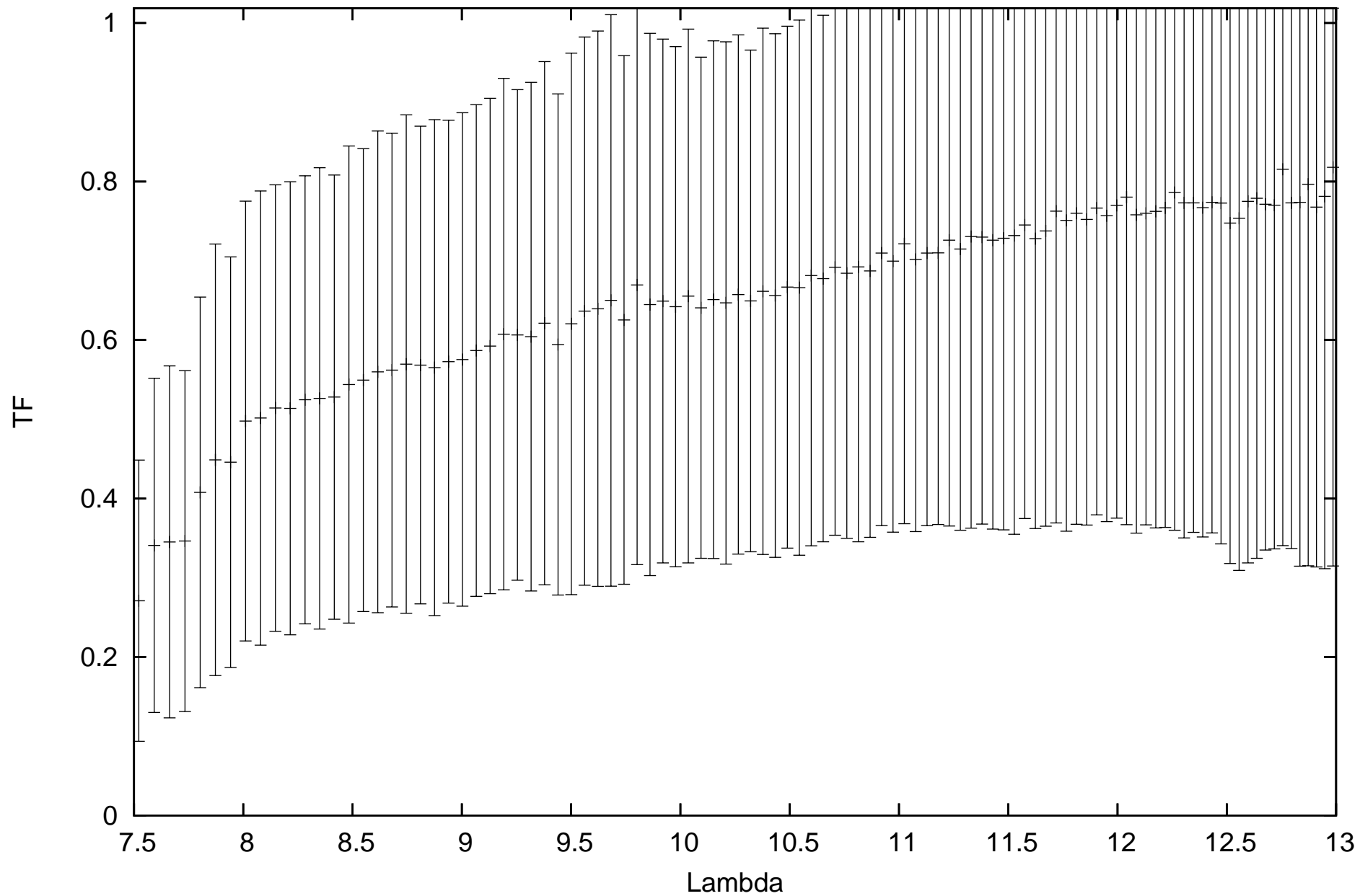
calHD023319_flux1.78_diam1.94_r.MIDI.2009-12-03T07_06_39.000_U2U4
