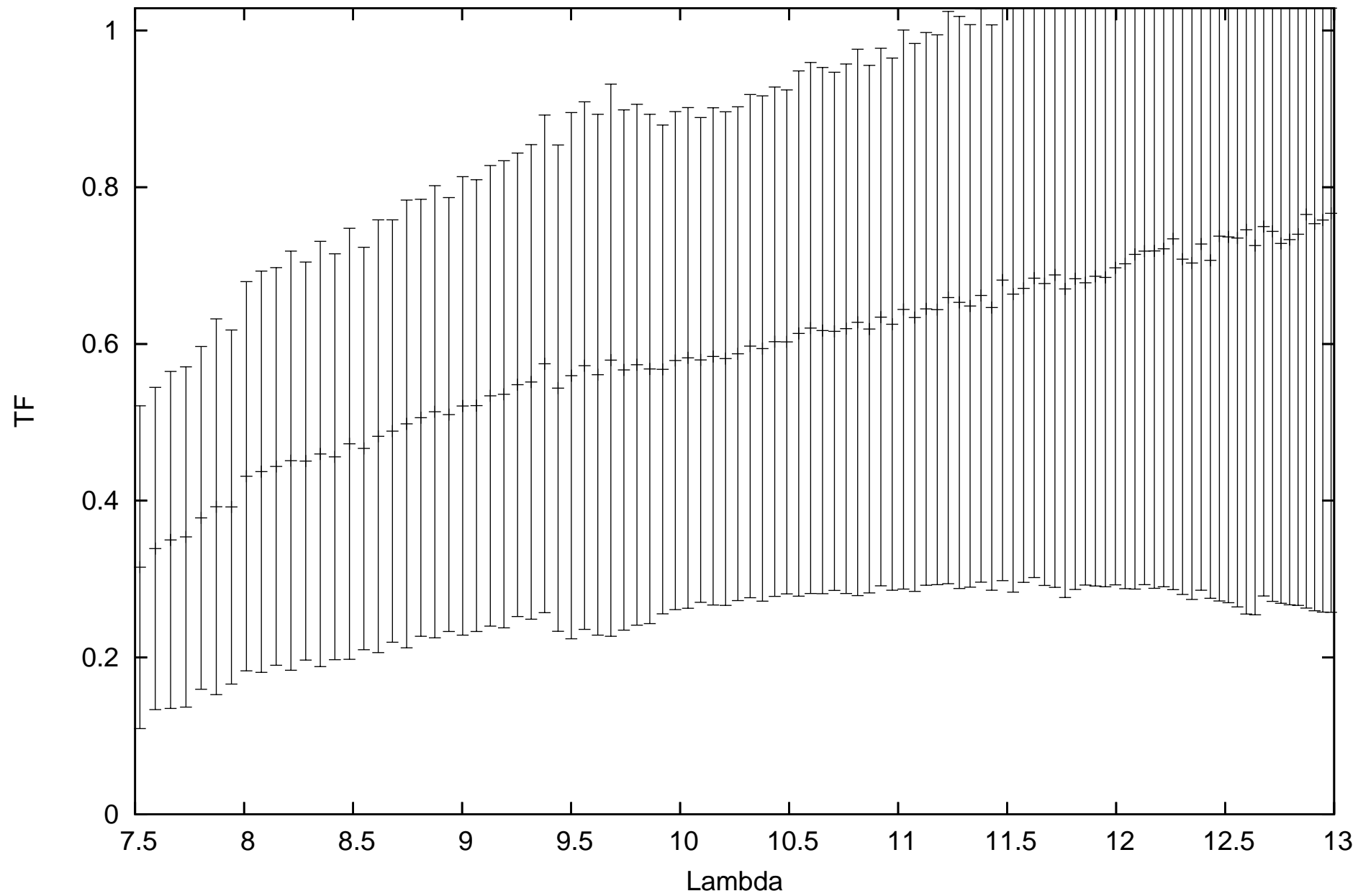
calHD039400_flux1.43_diam2.3_r.MIDI.2010-01-01T06_25_05.000_U3U4
