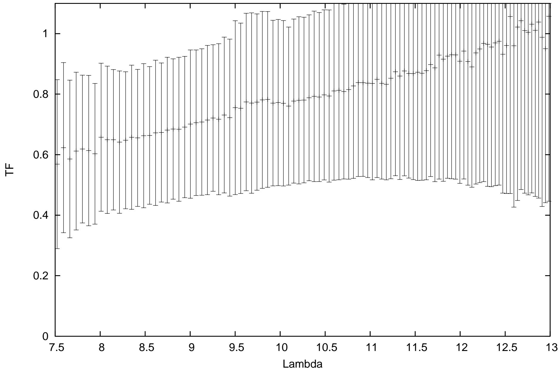
calHD031767_flux1.23_diam2.68_r.MIDI.2010-03-01T00_00_45.000_U1U2
