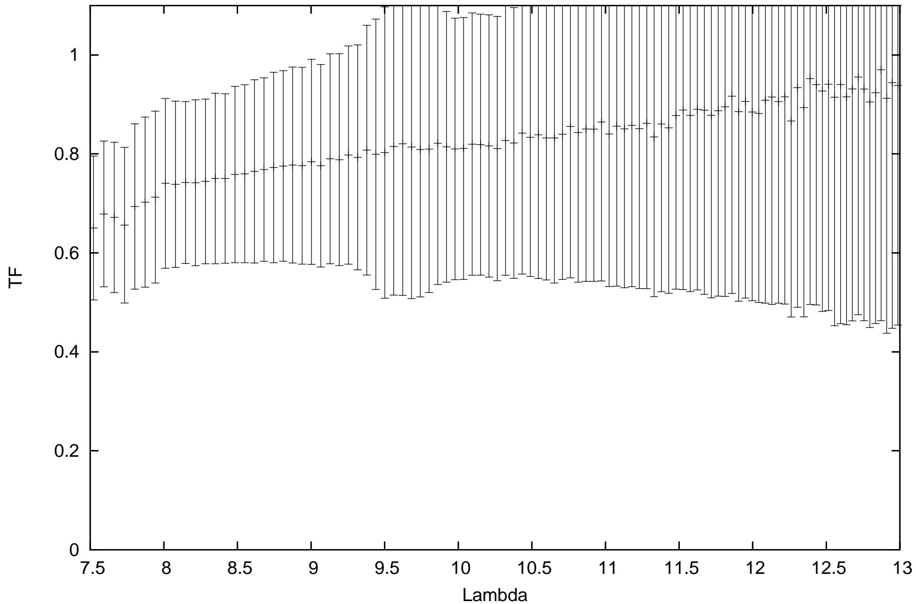
calHD126927_flux1.74_diam2.23_r.MIDI.2010-03-27T08_57_57.000_U1U2
