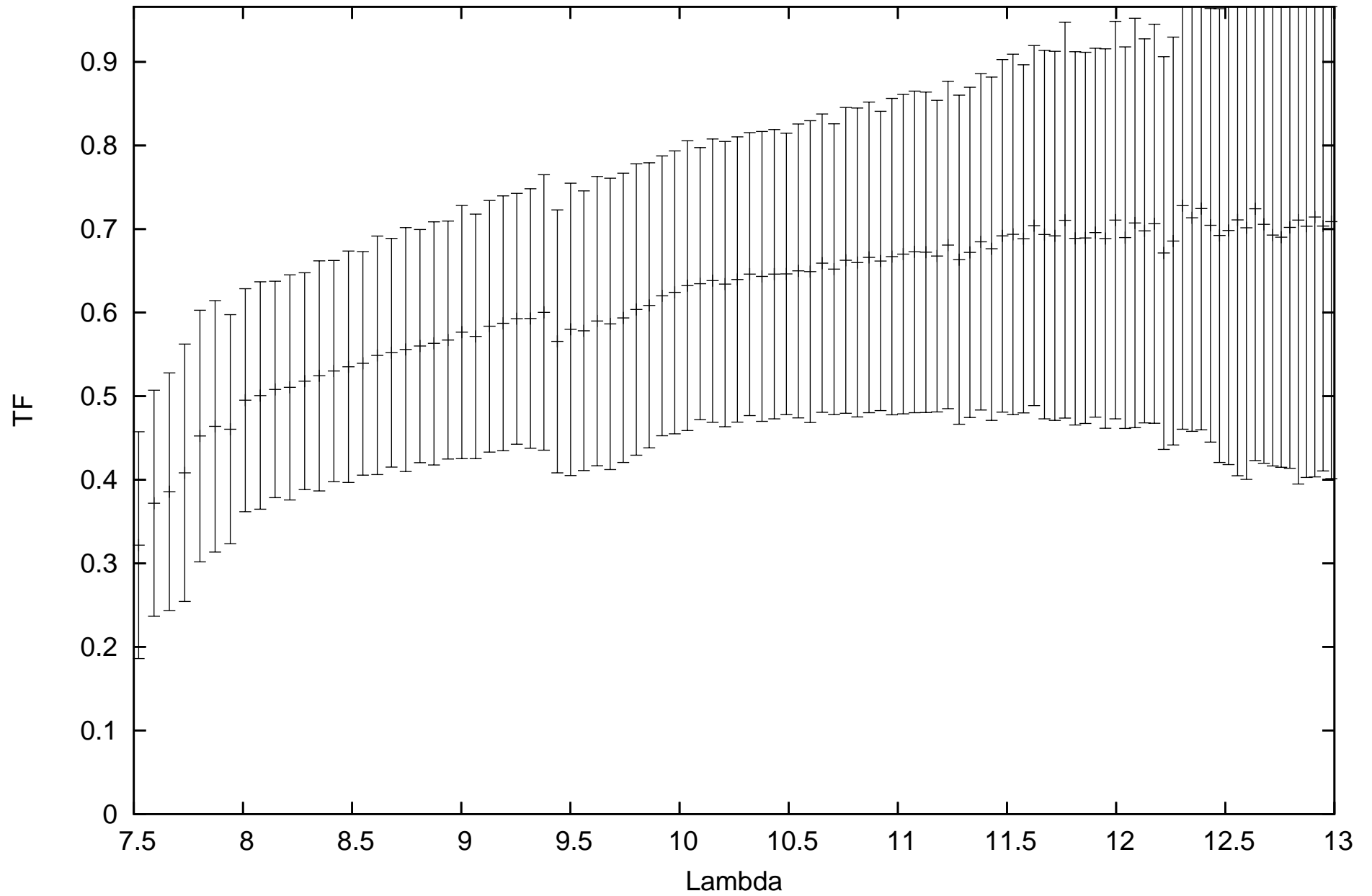
calHD081797_flux-1.49_diam9.14_r.MIDI.2010-04-02T03_41_01.000_K0A0
