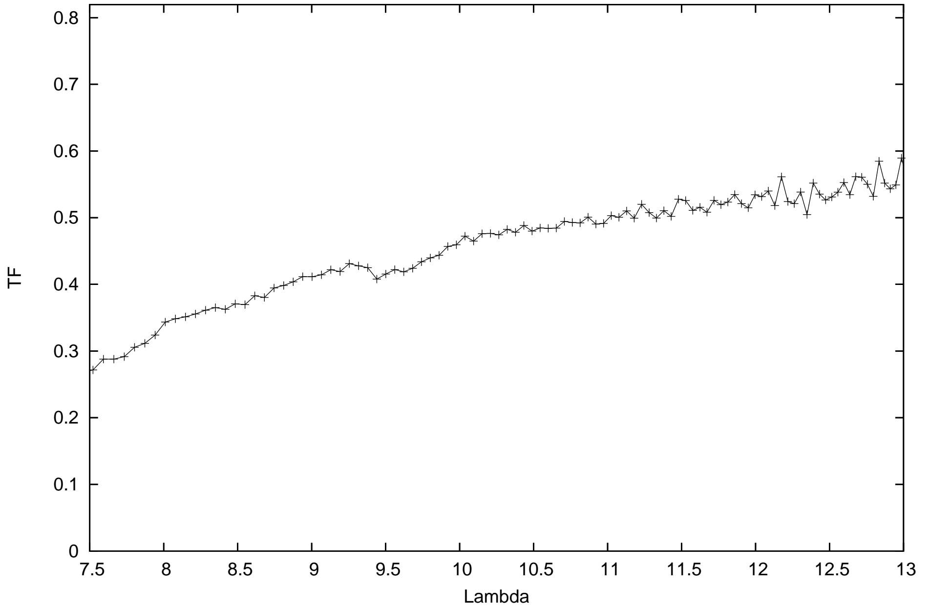
calHD081797_flux-1.49_diam9.14_r.MIDI.2010-05-22T22_57_17.000_H0E0
