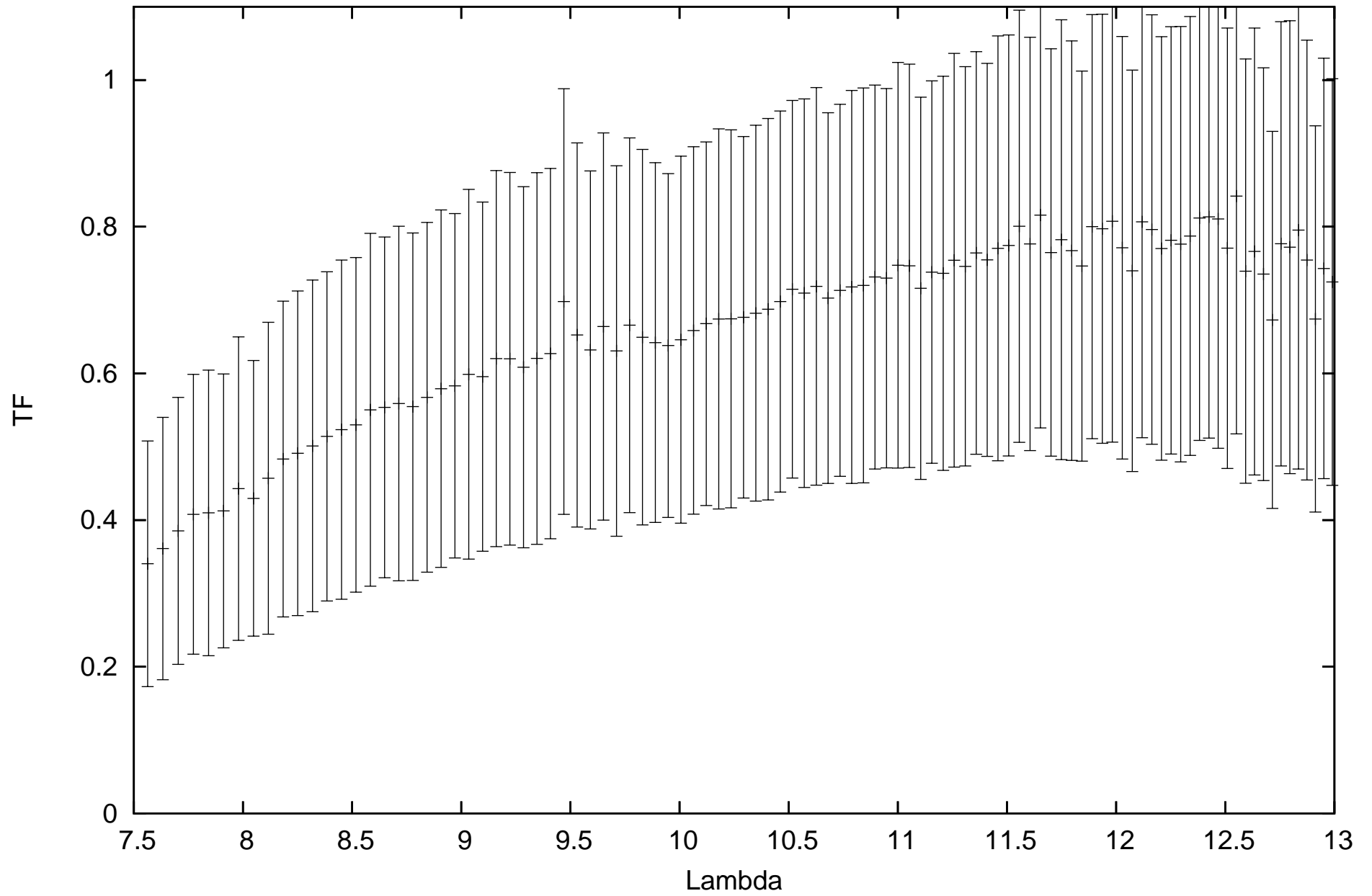
calHD120323_flux-2.02_diam13.25_r.MIDI.2010-06-07T02_42_16.686_H0E0
