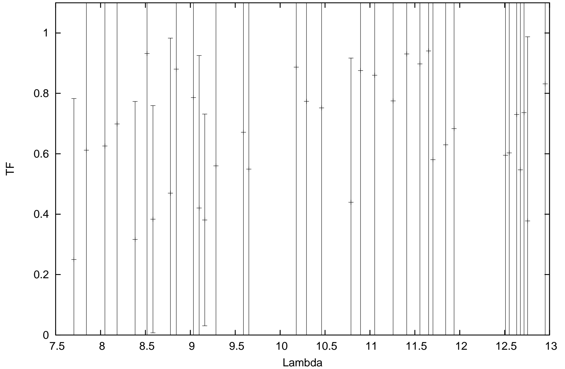
calHD216386_flux-0.89_diam7.58_r.MIDI.2010-06-23T10_08_58.945_K0G1
