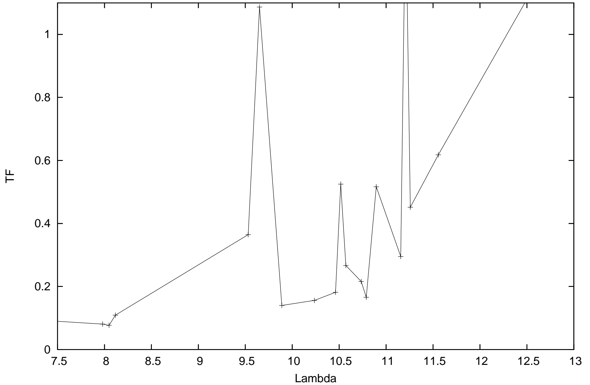
calHD133216_flux-1.76_diam11.15_r.MIDI.2010-07-08T02_33_34.138_I1D0
