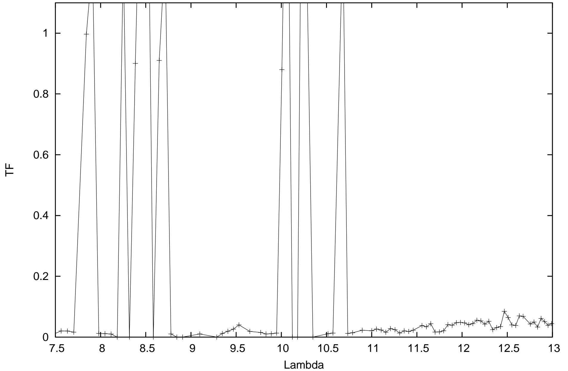
calHD133216_flux-1.76_diam11.15_r.MIDI.2010-07-08T03_14_45.110_I1D0
