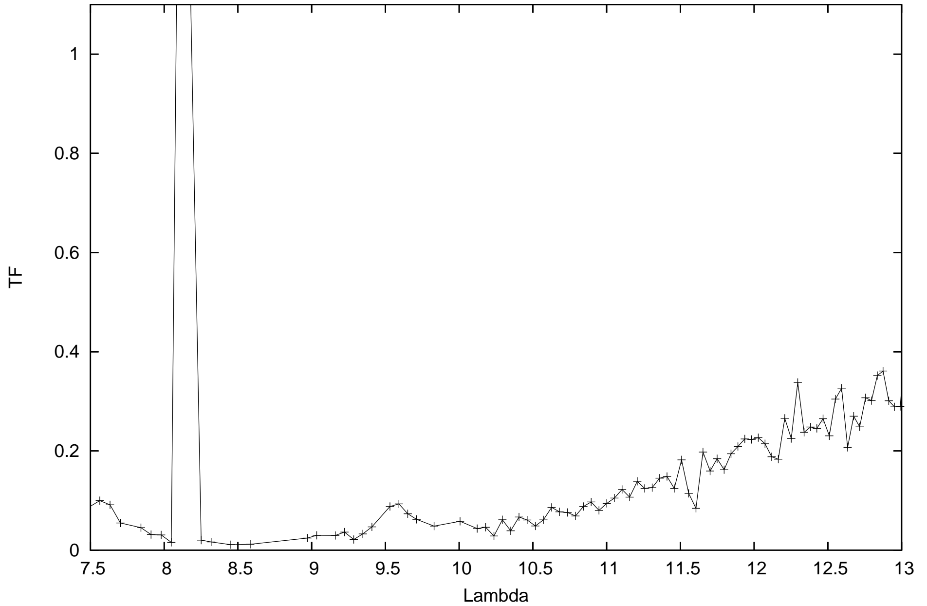
calHD133216_flux-1.76_diam11.15_r.MIDI.2010-07-08T03_38_08.123_I1D0
