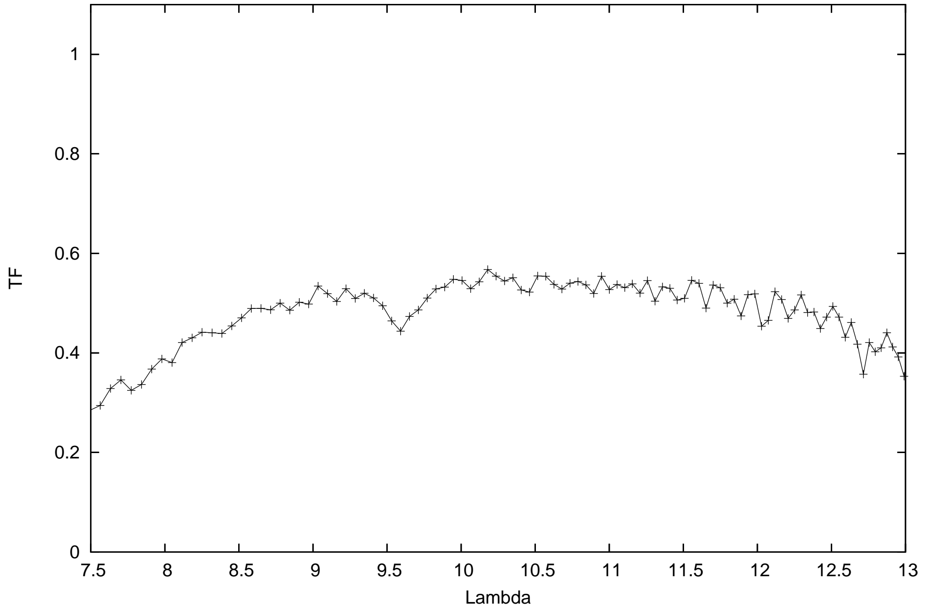
calHD167618_flux-1.82_diam11.66_r.MIDI.2010-07-14T05_44_25.137_H0I1
