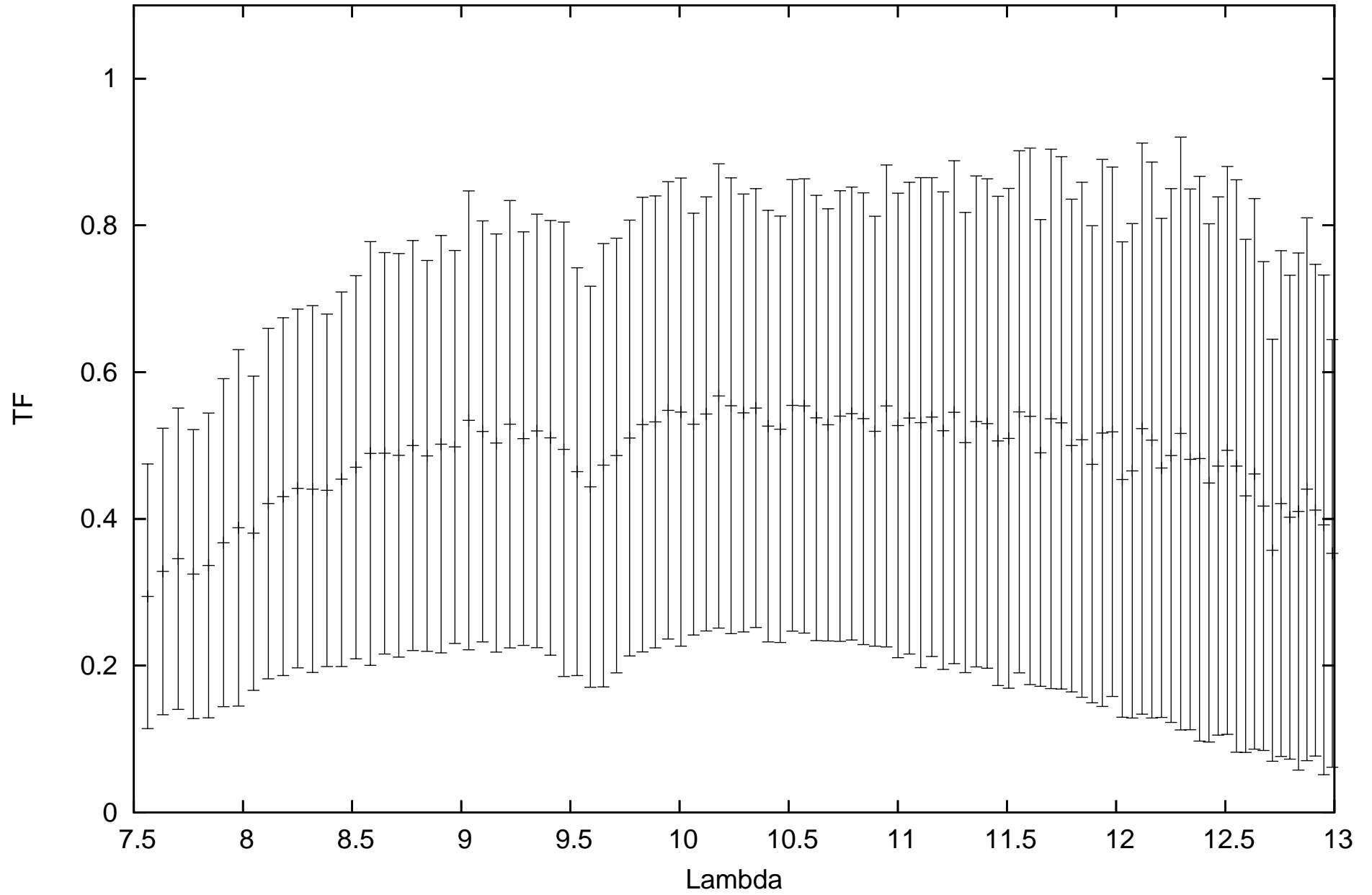
calHD167618_flux-1.82_diam11.66_r.MIDI.2010-07-14T05_44_25.137_H011
