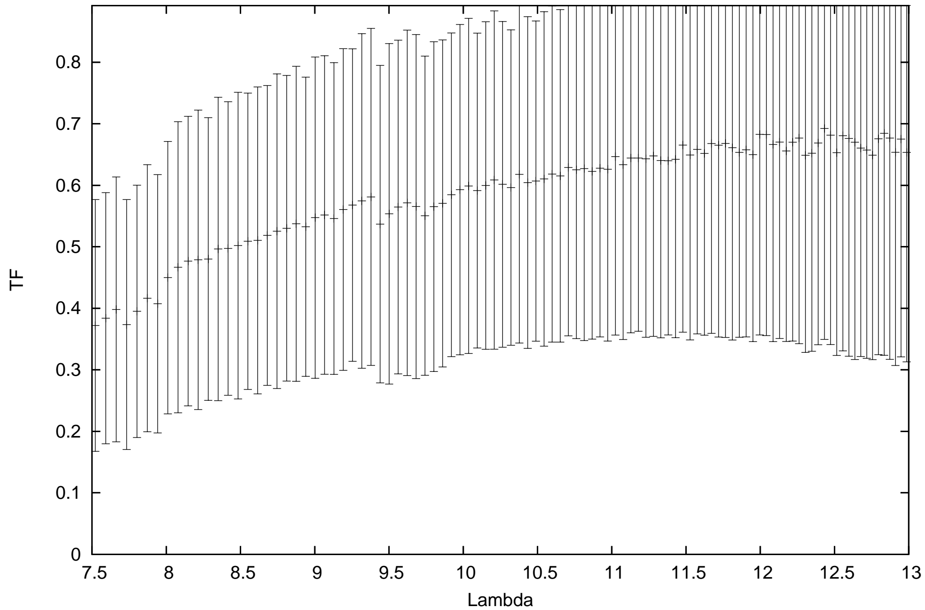
calHD009138_flux1.4_diam2.55_r.MIDI.2010-08-25T06_49_02.000_U1U2
