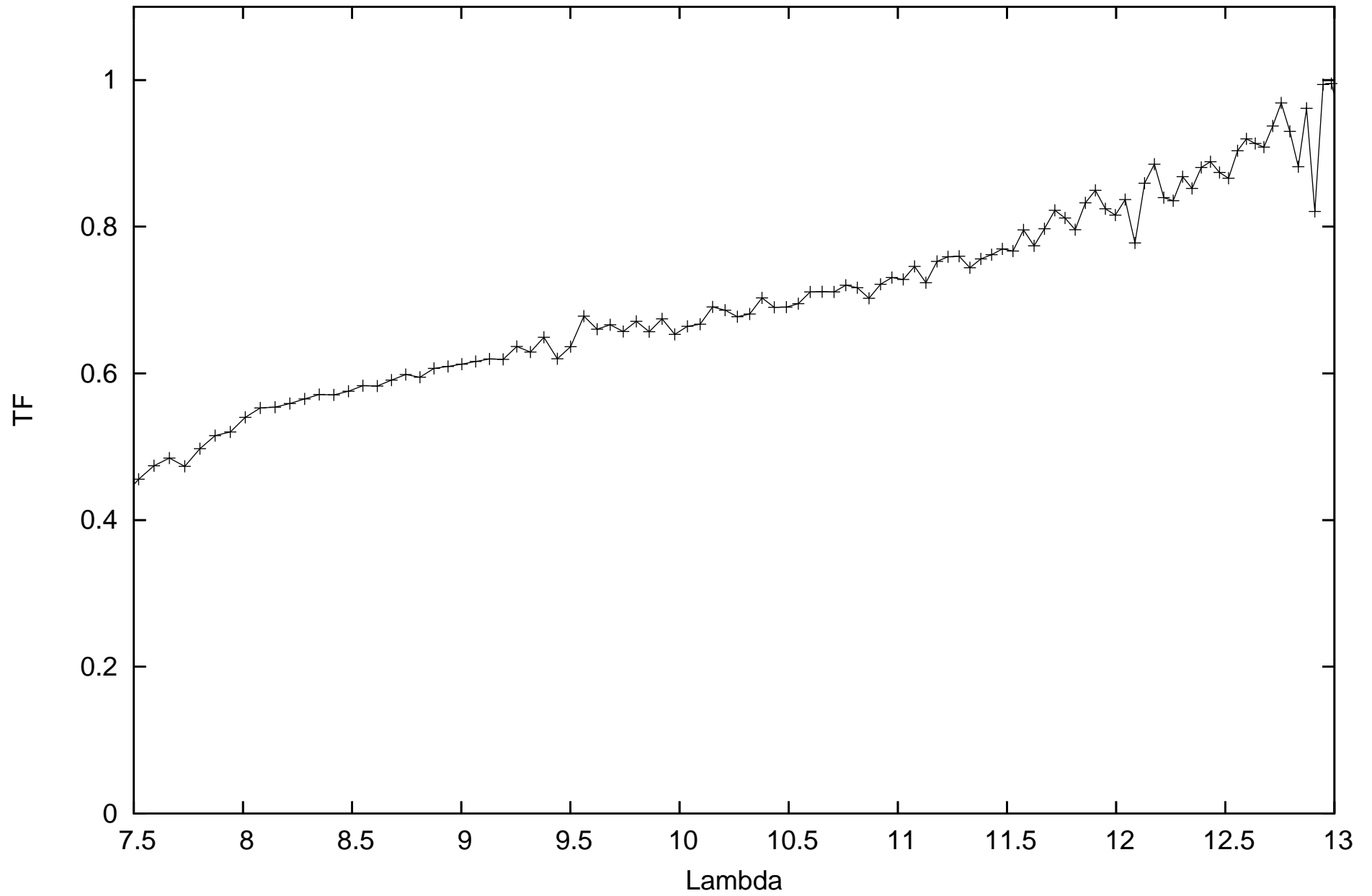
calHD023319_flux1.78_diam1.94_r.MIDI.2010-08-25T09_36_38.000_U1U2
