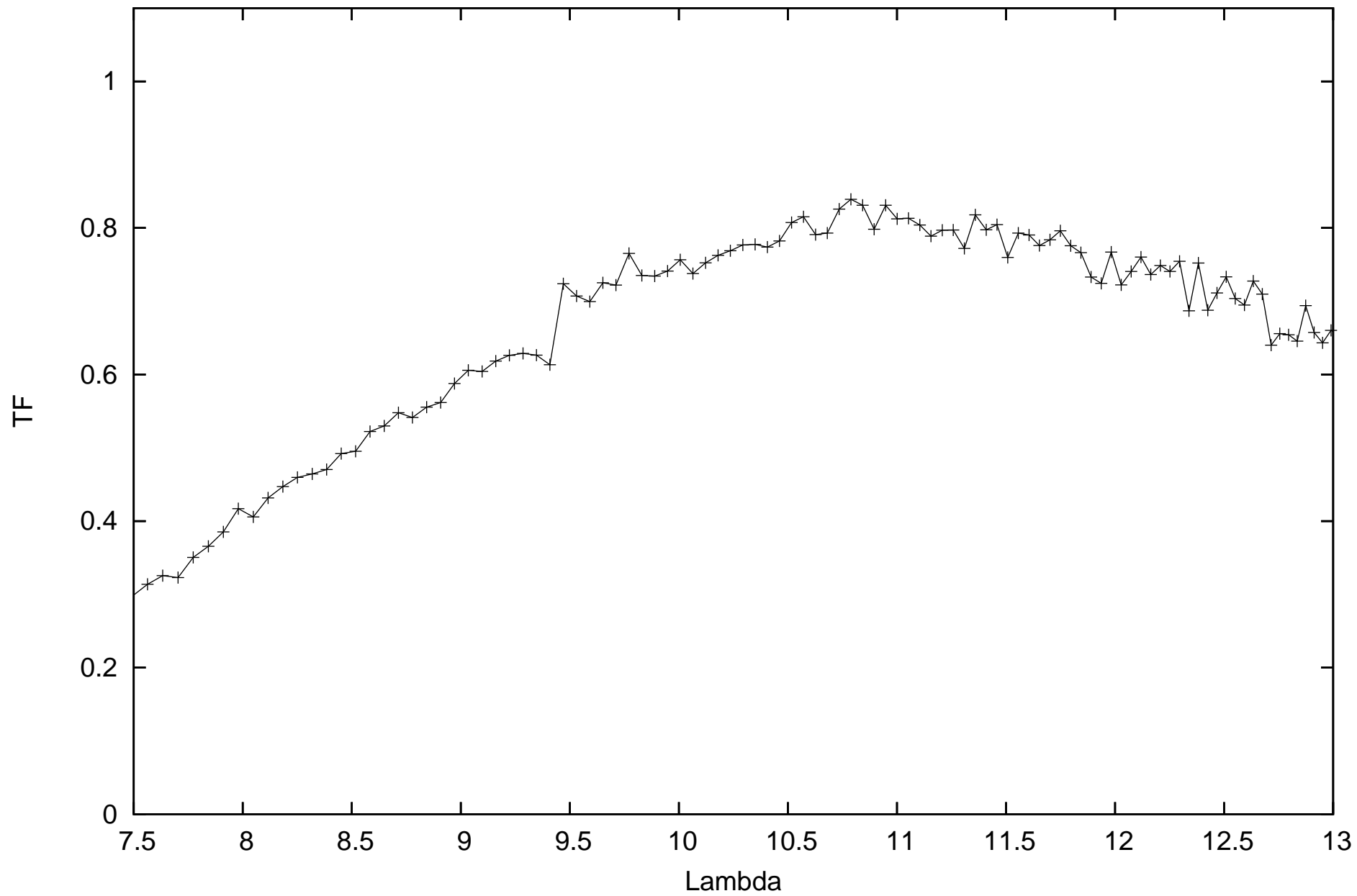
calHD167618_flux-1.82_diam11.66_r.MIDI.2010-08-25T04_28_51.973_U1U2
