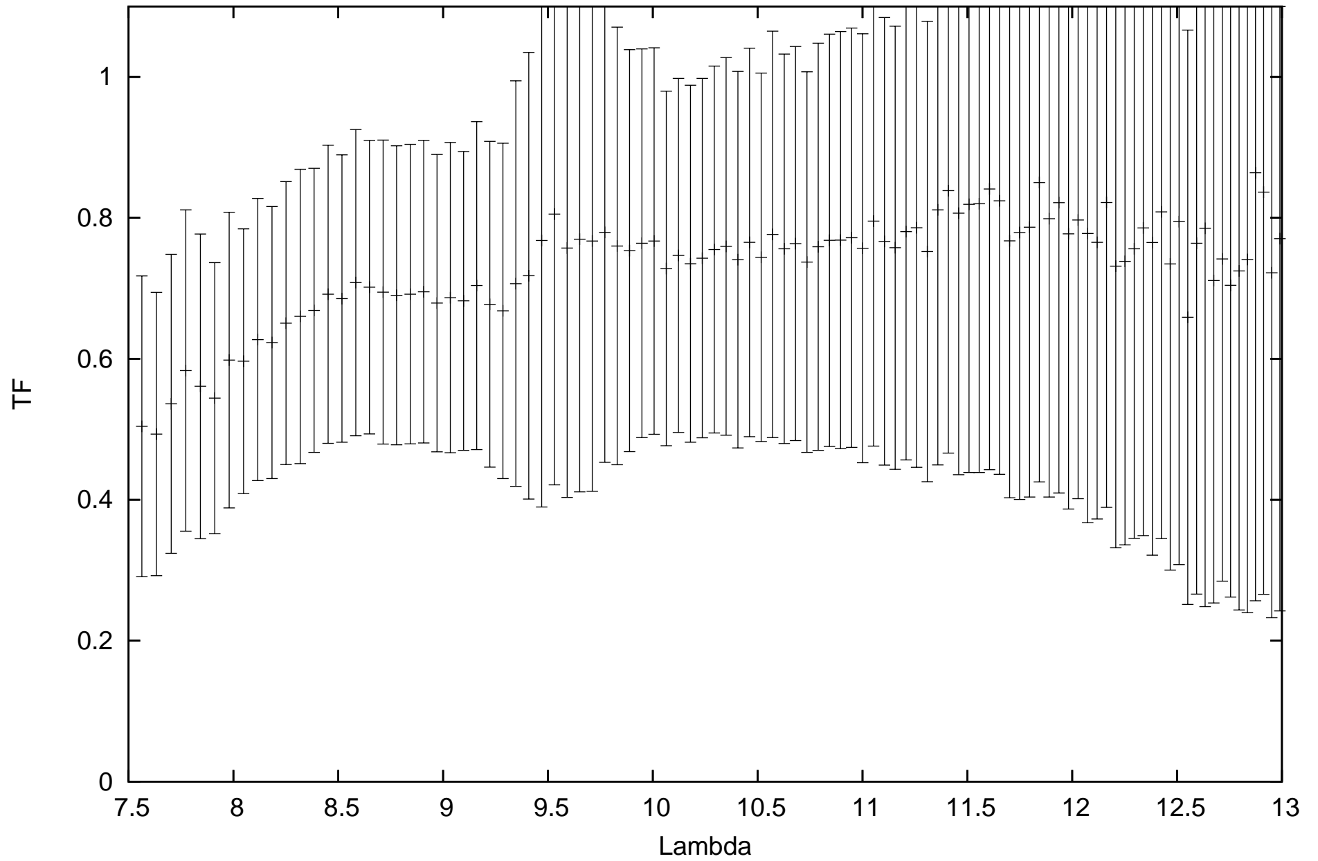
calHD081797_flux-1.49_diam9.14_r.MIDI.2011-01-11T07_31_19.138_D0A1
