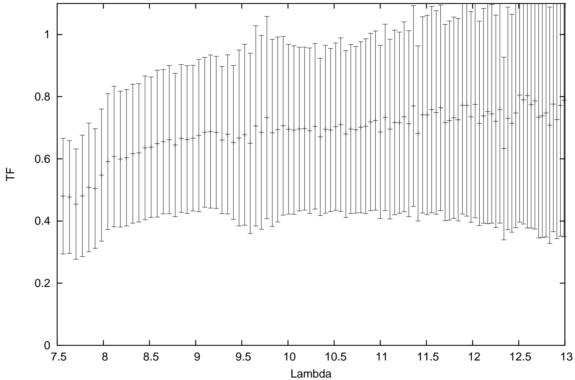
calHD120404_flux1.19_diam2.96_r.MIDI.2011-01-17T07_43_35.781_U2U3
