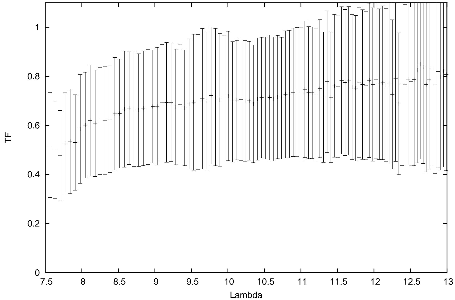
calHD120404_flux1.19_diam2.96_r.MIDI.2011-01-17T07_50_41.946_U2U3
